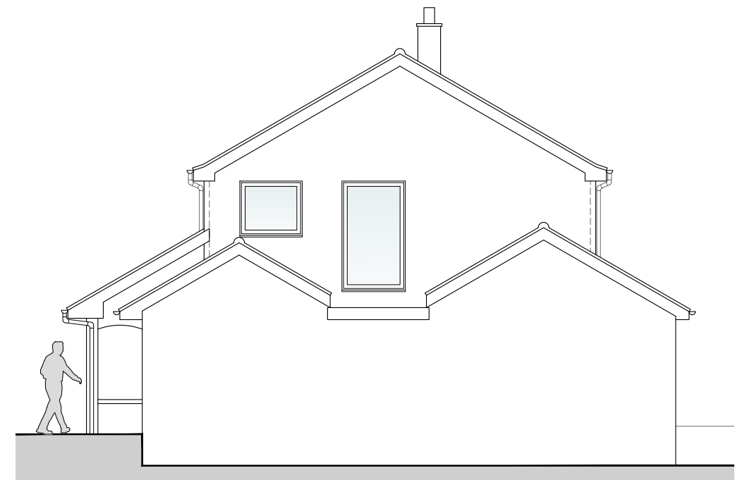
EXISTING WEST ELEVATION 1:100@A3
