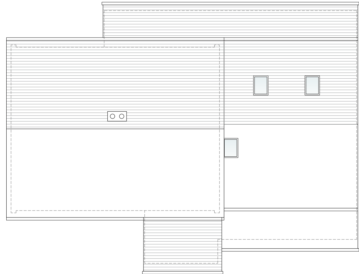
PROPOSED ROOF PLAN 1:100@A3
