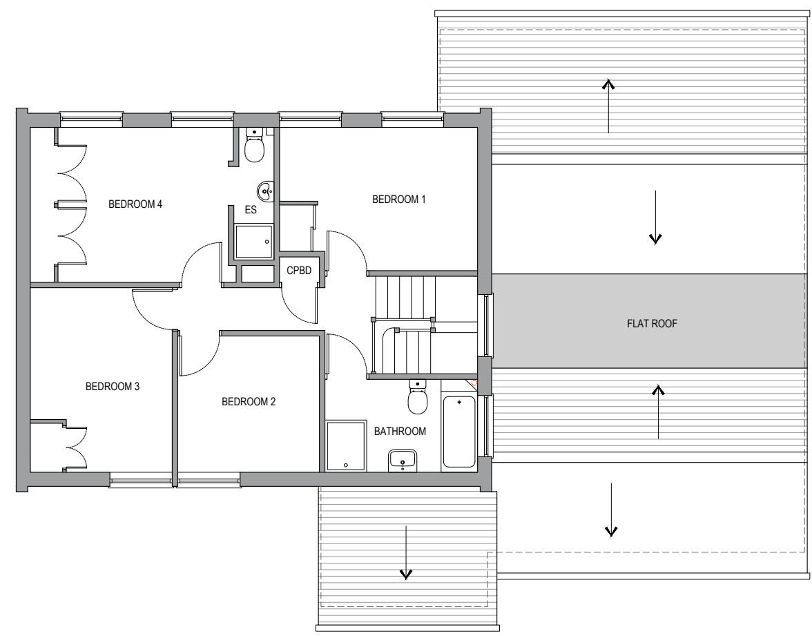
EXISTING FIRST FLOOR PLAN 1:100@A3
