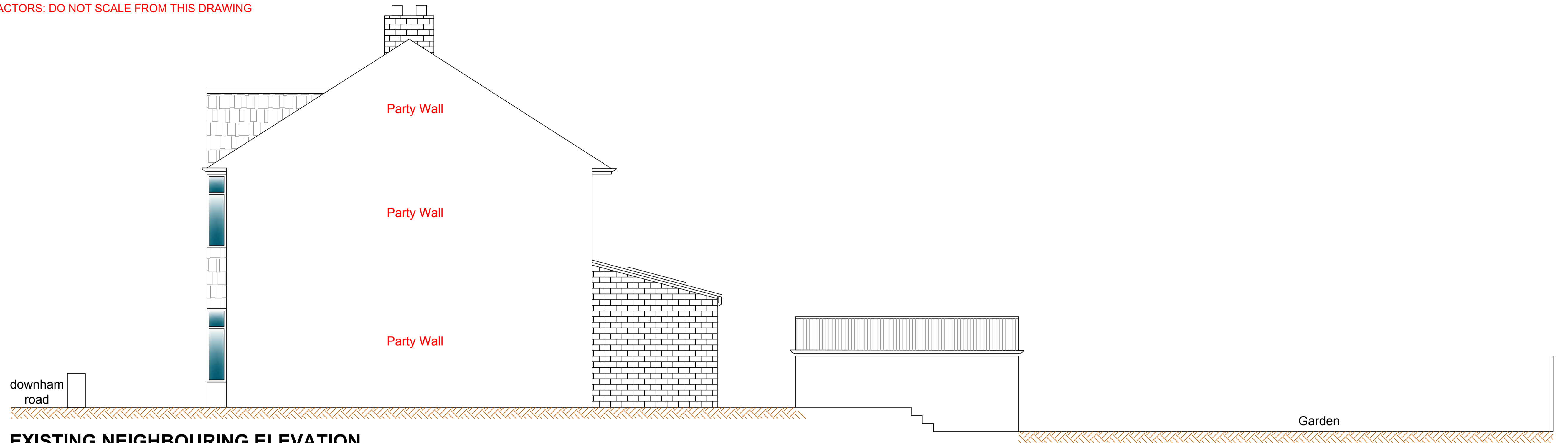
EXISTING NEIGHBOURING ELEVATION 1:50 @ A1
