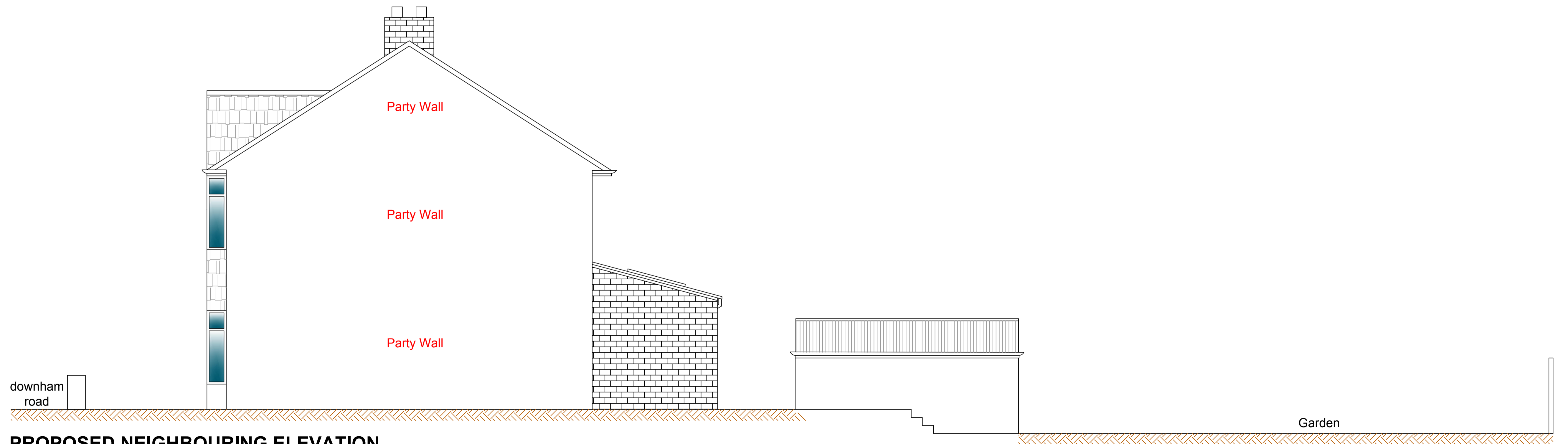
PROPOSED NEIGHBOURING ELEVATION 1:50 @ A1
