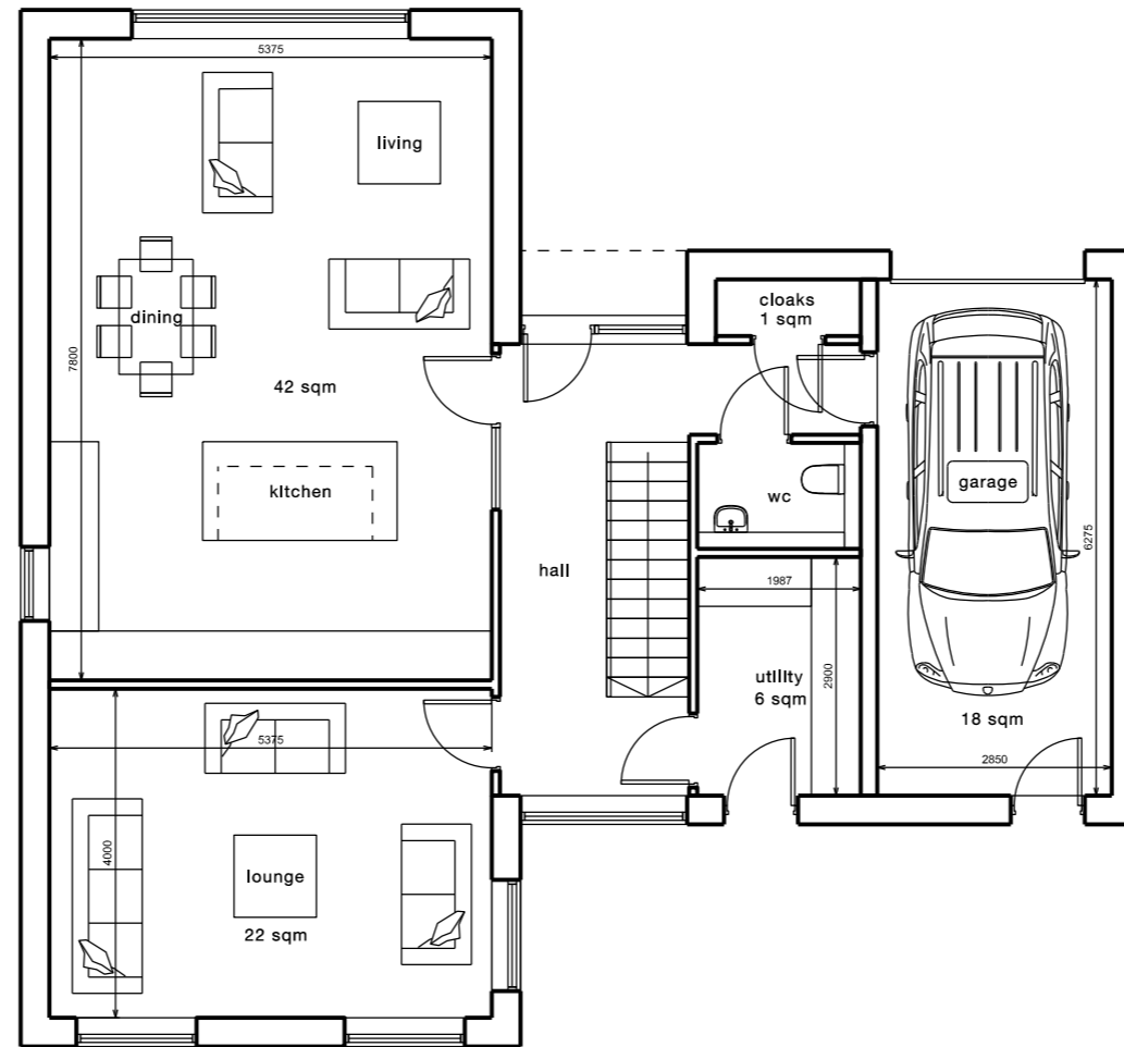
ground floor GIA 109 sqm
