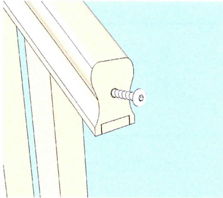
Raking handrail mechanical fixings
