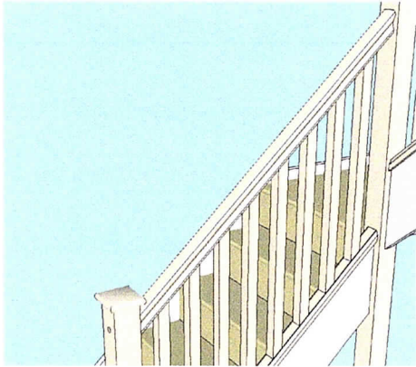
Raking handrails pre-cut
