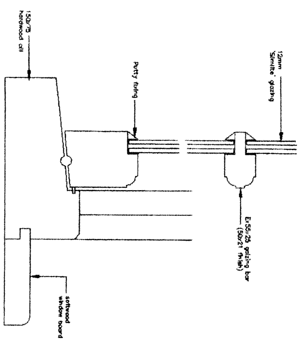
Vertical Section - 'Simlilite' Glazing 1:2
