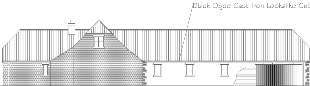
North Elevation
