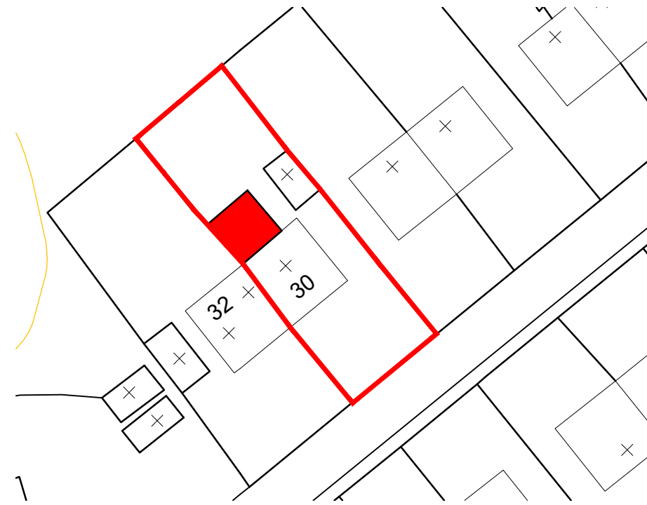
Site Block Plan As Proposed 1:500
