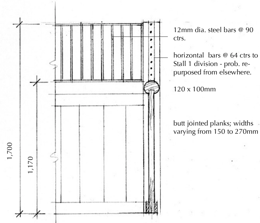
DETAIL OF STALL DIVISION 1:20
