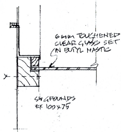
SIDE SECTION
