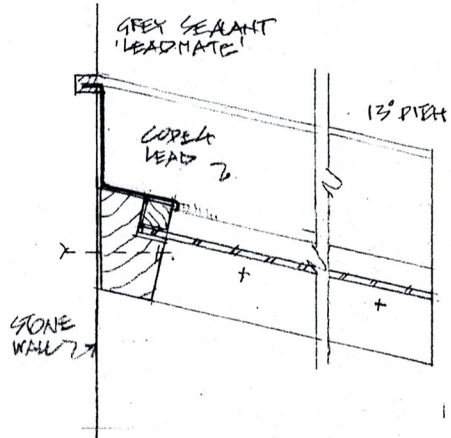
SECTION AT TOP
