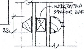
SECTION 1:2 DETAIL A
