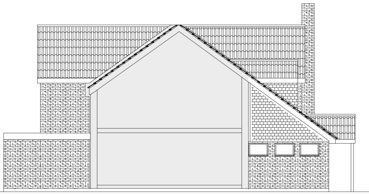
side (S) elevation
