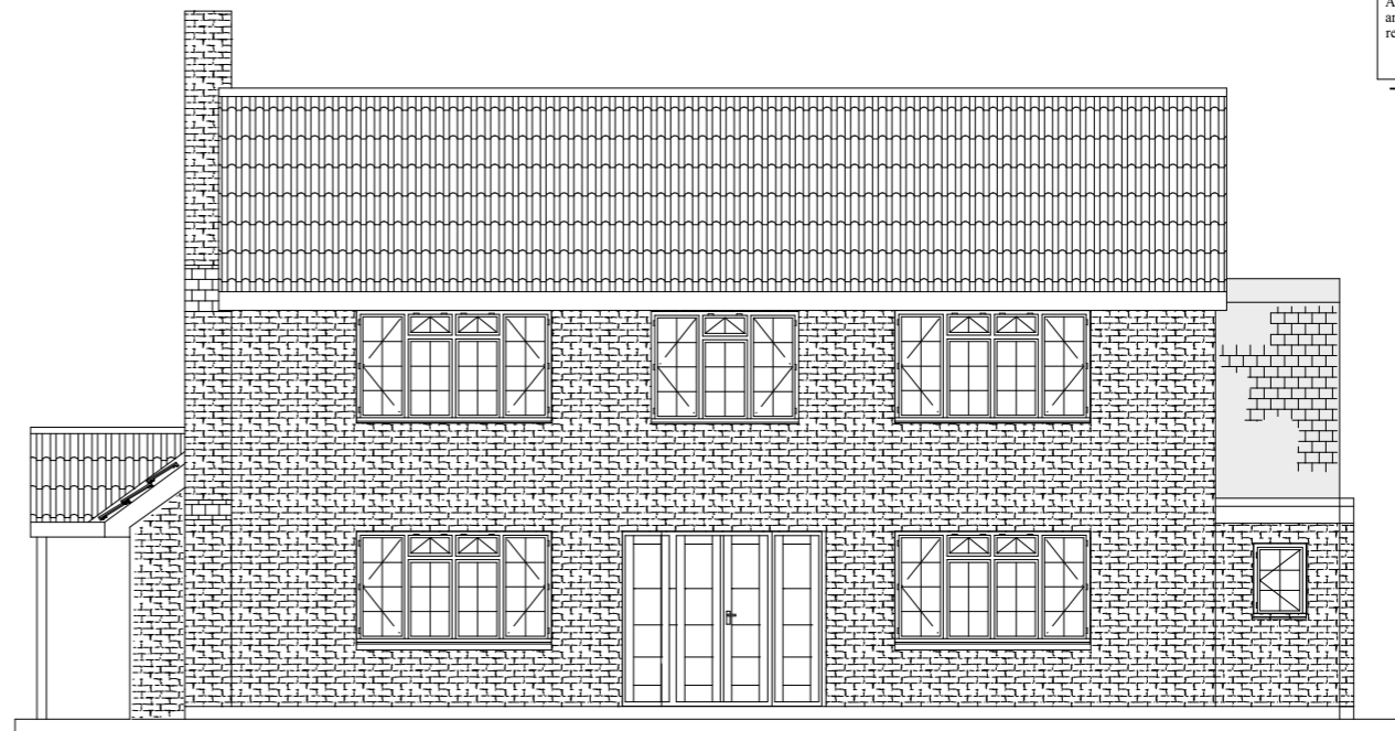
side (N) elevation
