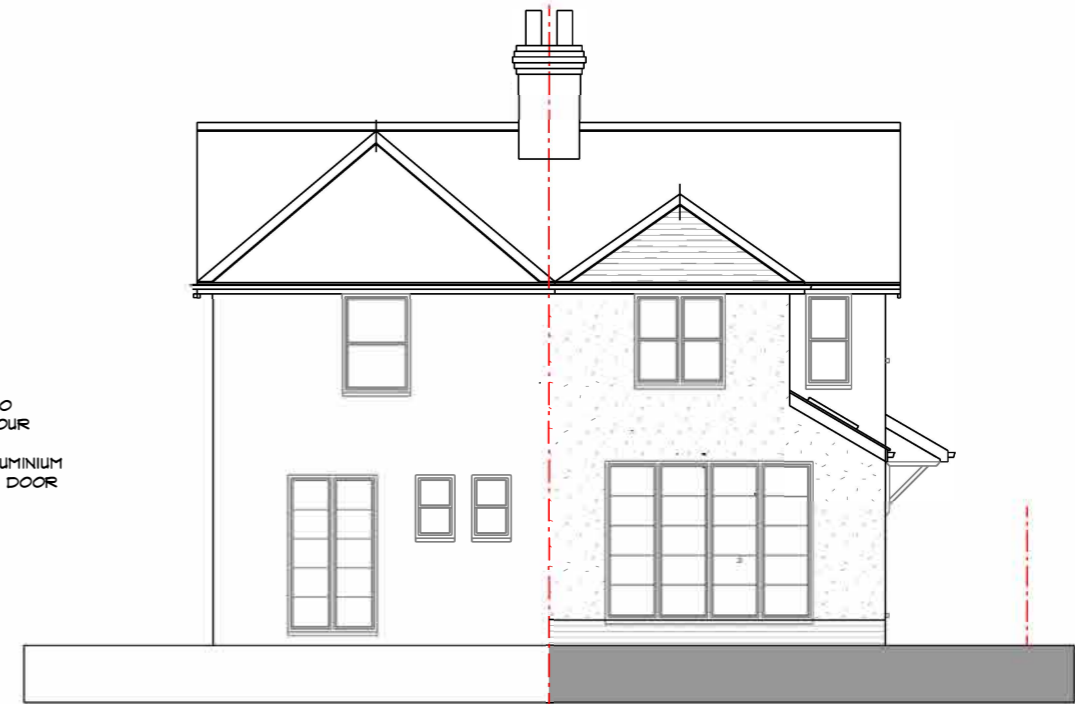
PROPOSED REAR ELEVATION - NORTH Scale 1:100 @ A3
