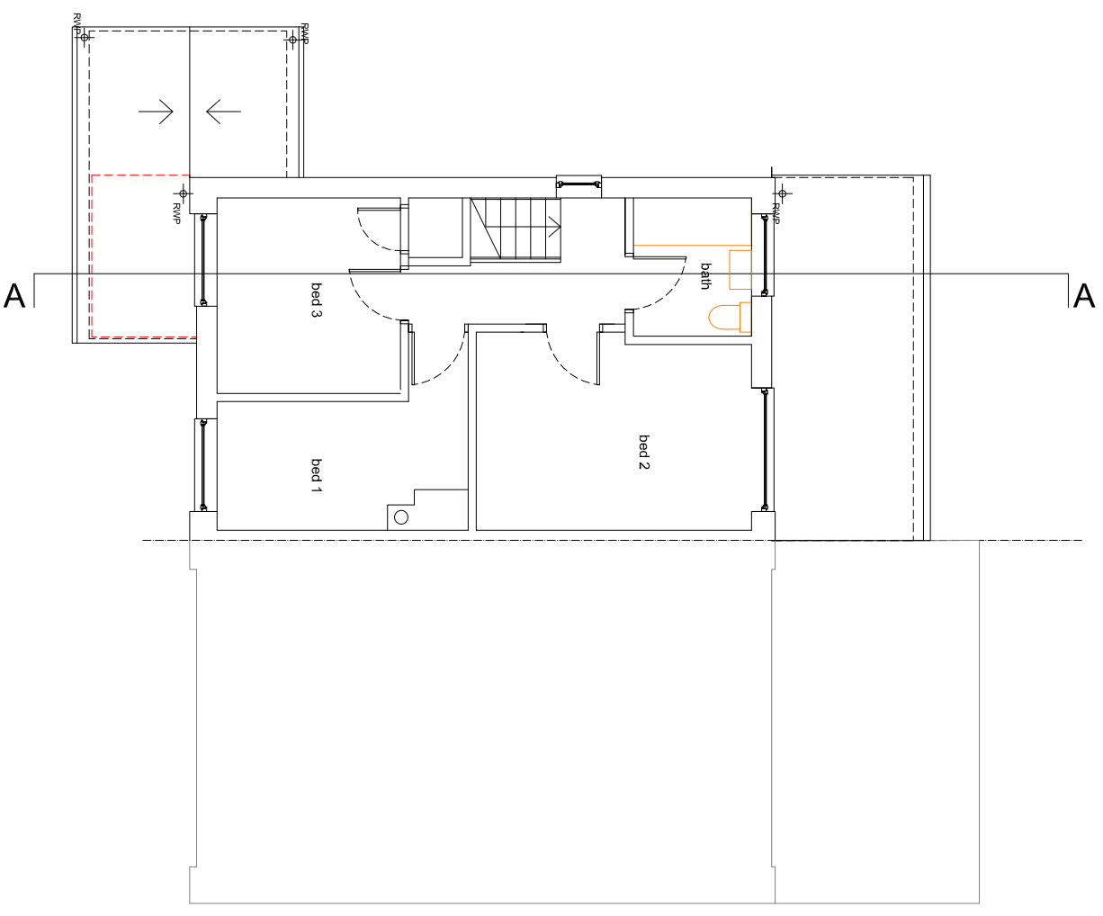
proposed-upper floor porch-roof
