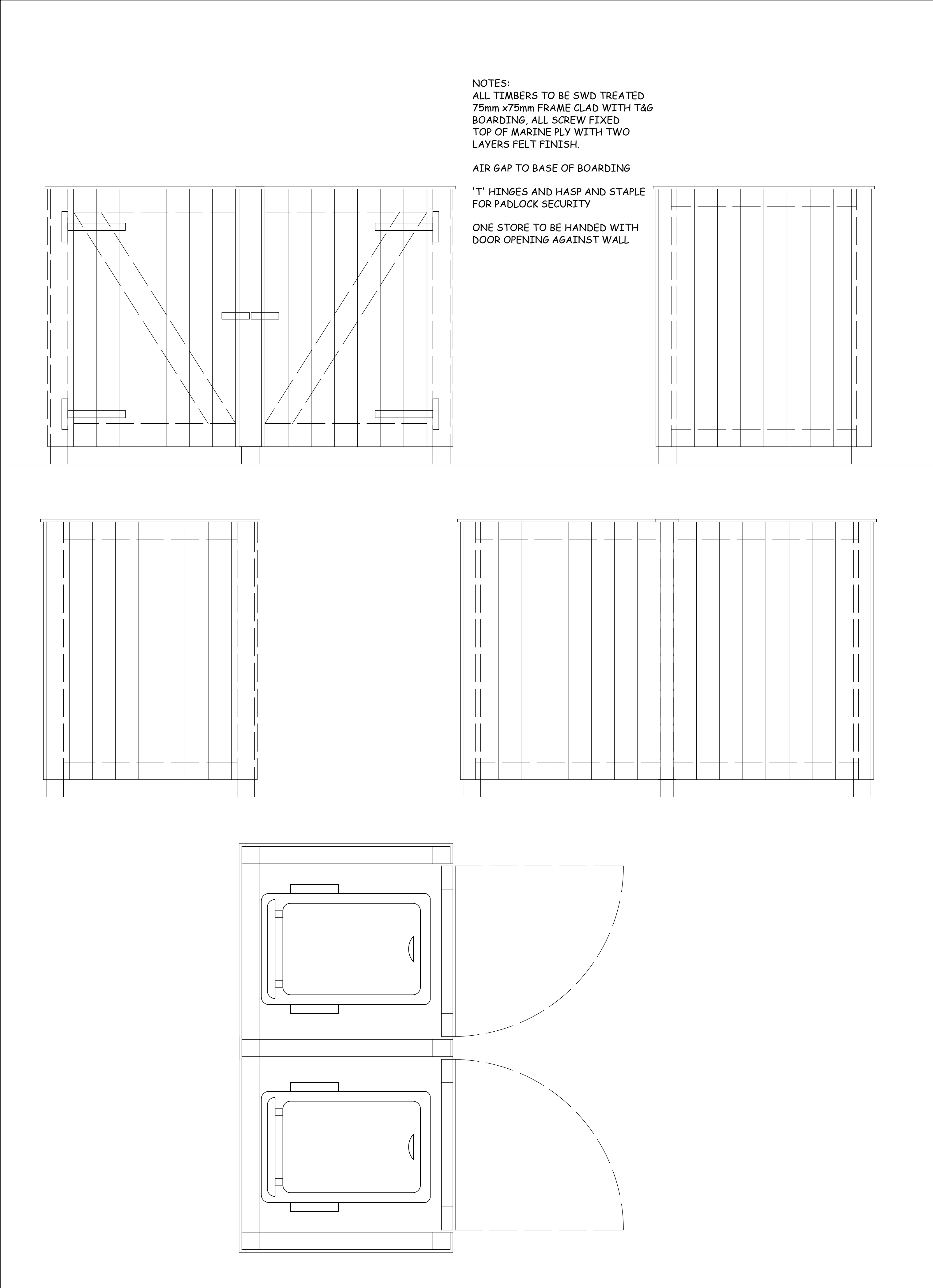
BIN STORE SCALE 1/10
