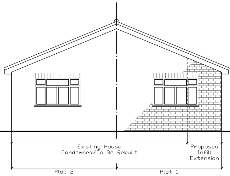
1:100 Proposed Front Elevation
