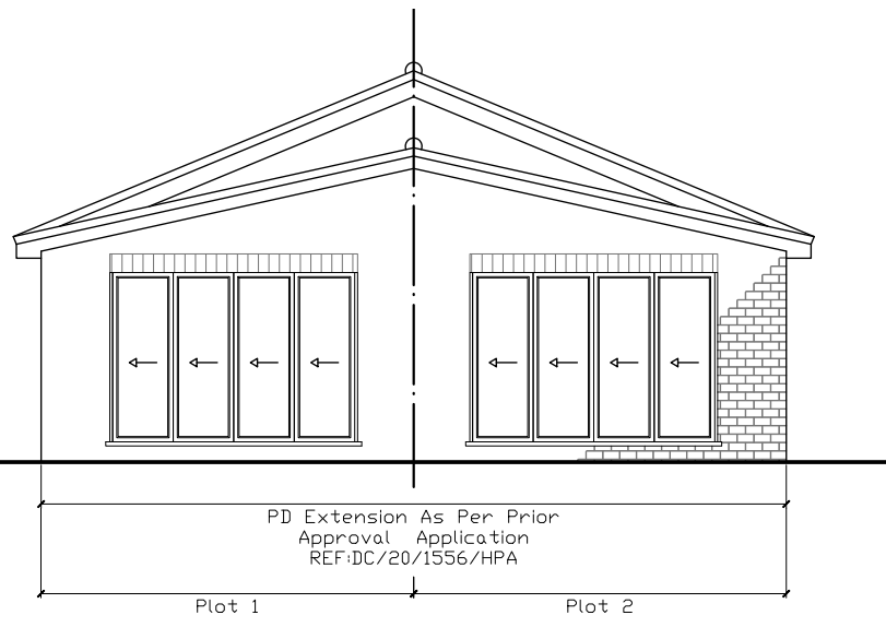
1:100 Proposed Rear Elevation
