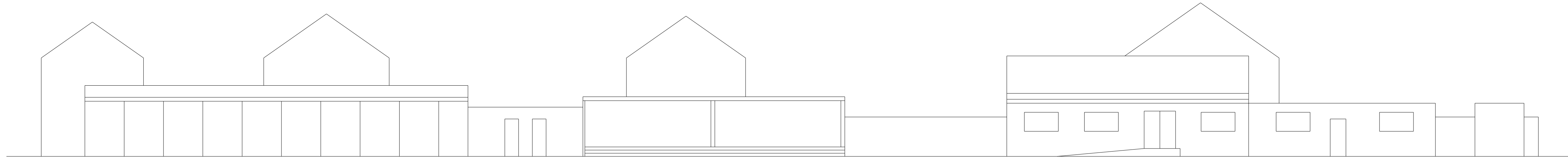
Club House View From Pitch scale 1:100
