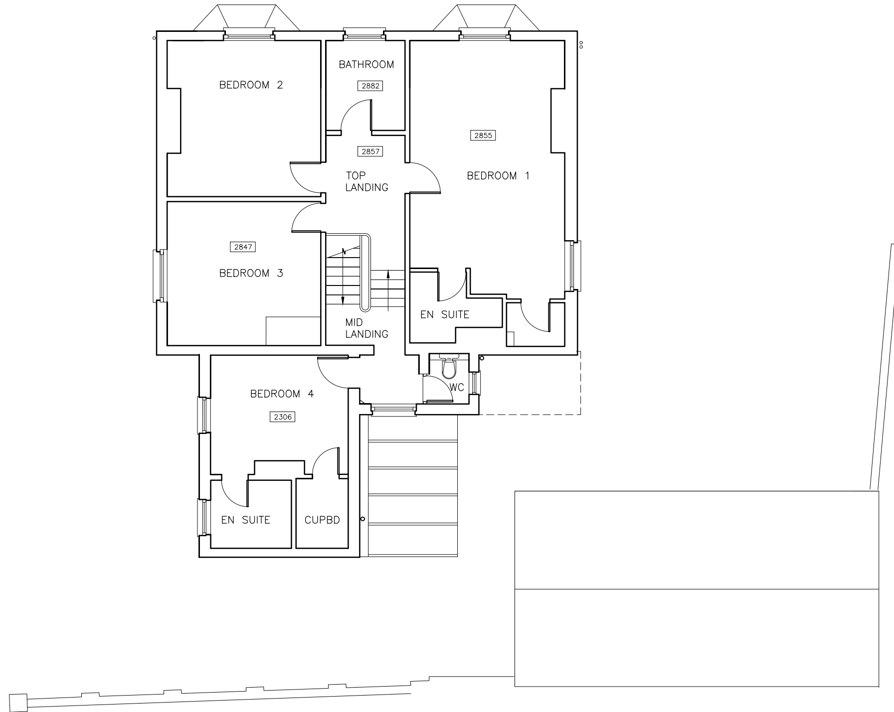
EXISTING FIRST FLOOR LAYOUT
