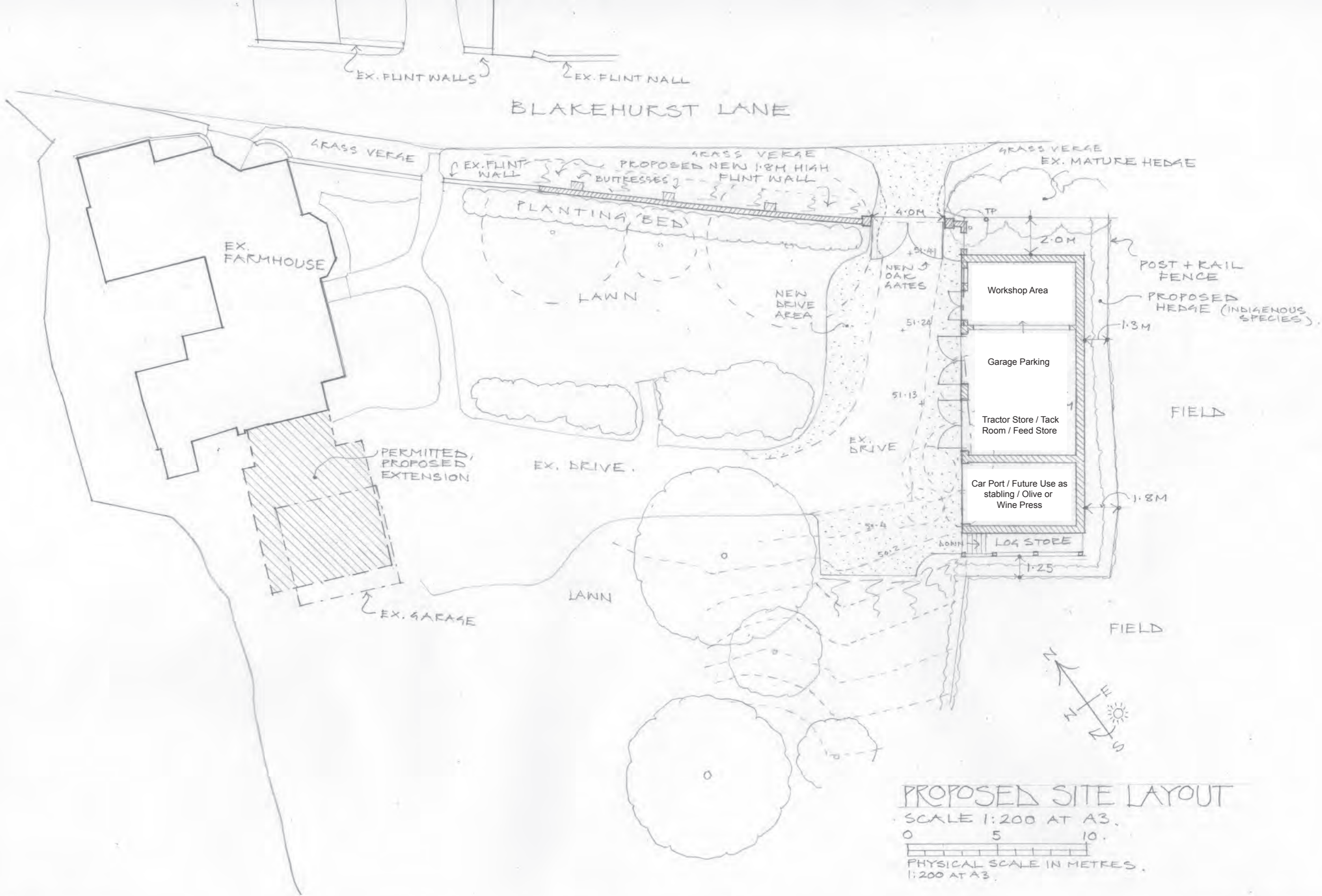
A PROPOSED BOUNDARY WALL & GARAGE/WORKSHOP AT WARNINGCAMP FARMHOUSE BLAKEHURST LANE, WARNINGCAMP JOB NO. 1457 DRWG. NO. 402 © 18th OCTOBER 2021
