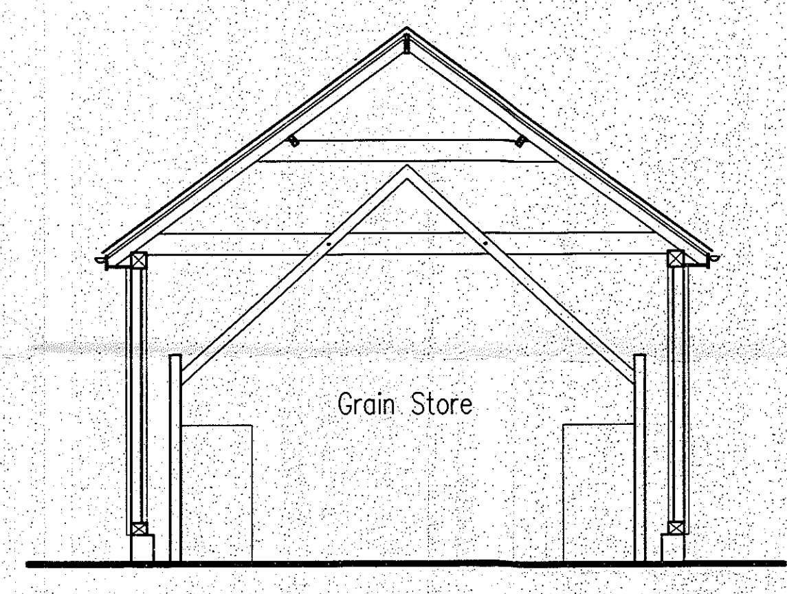
SECTION 1/50 @ A1
