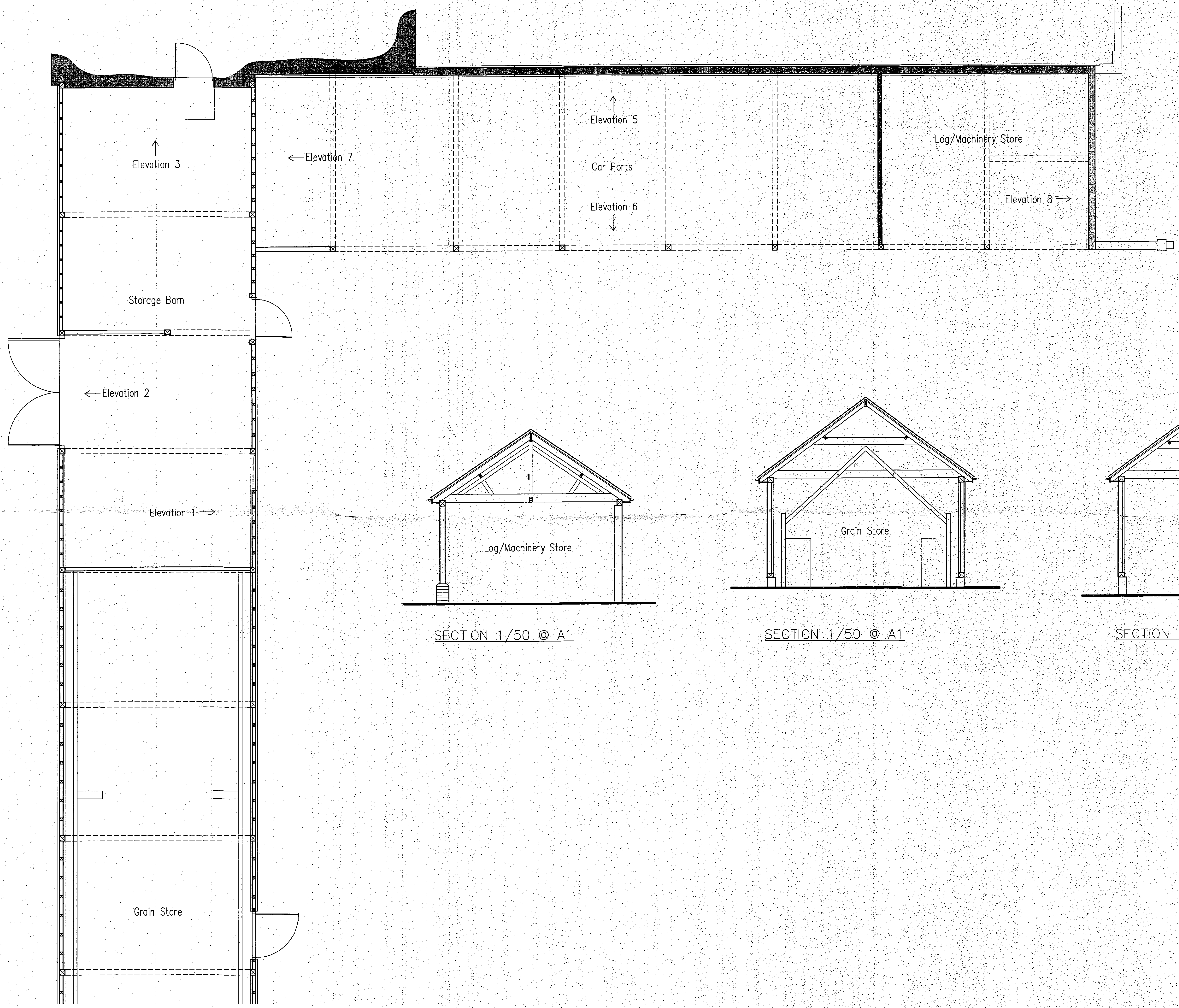
GROUND FLOOR PLAN 1/50 @ A1
