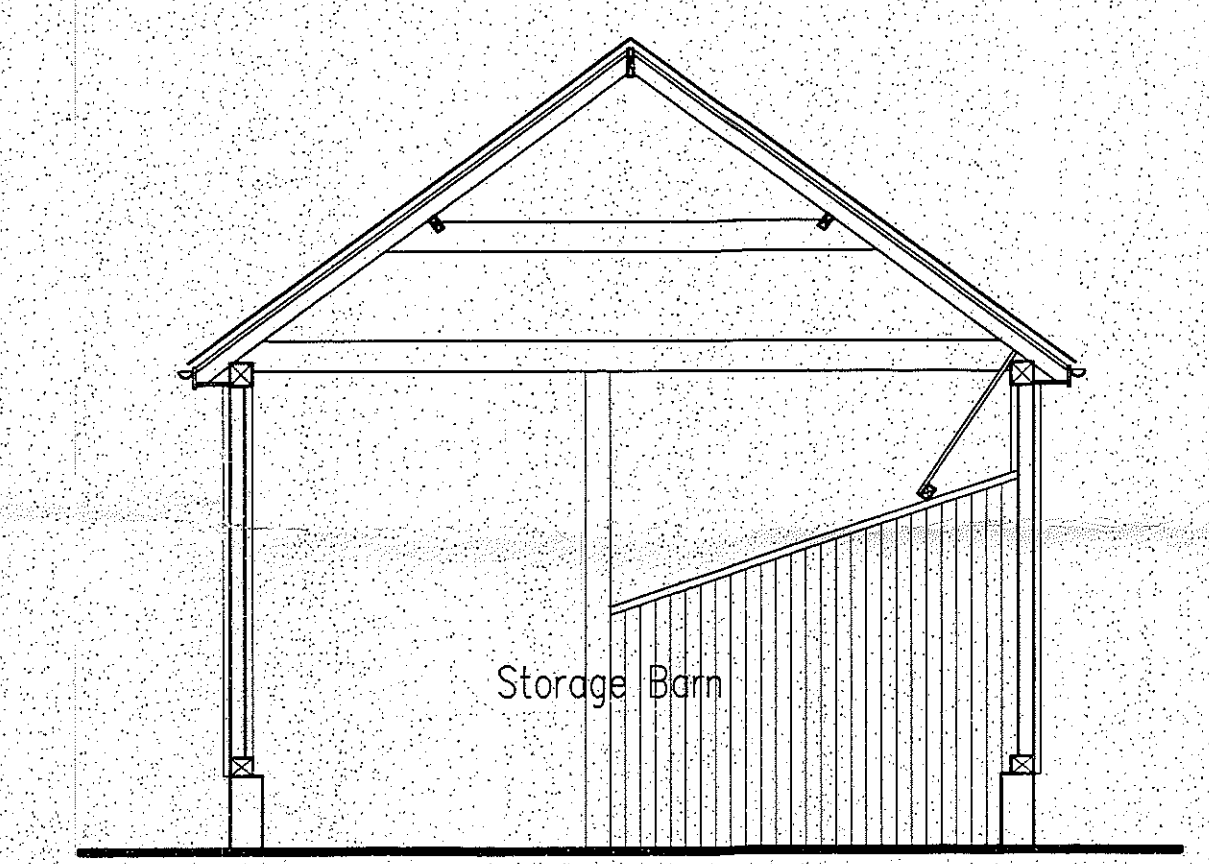
SECTION 1/50 @ A1
