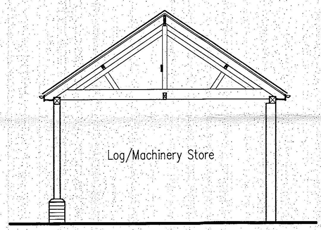
SECTION 1/50 @ A1
