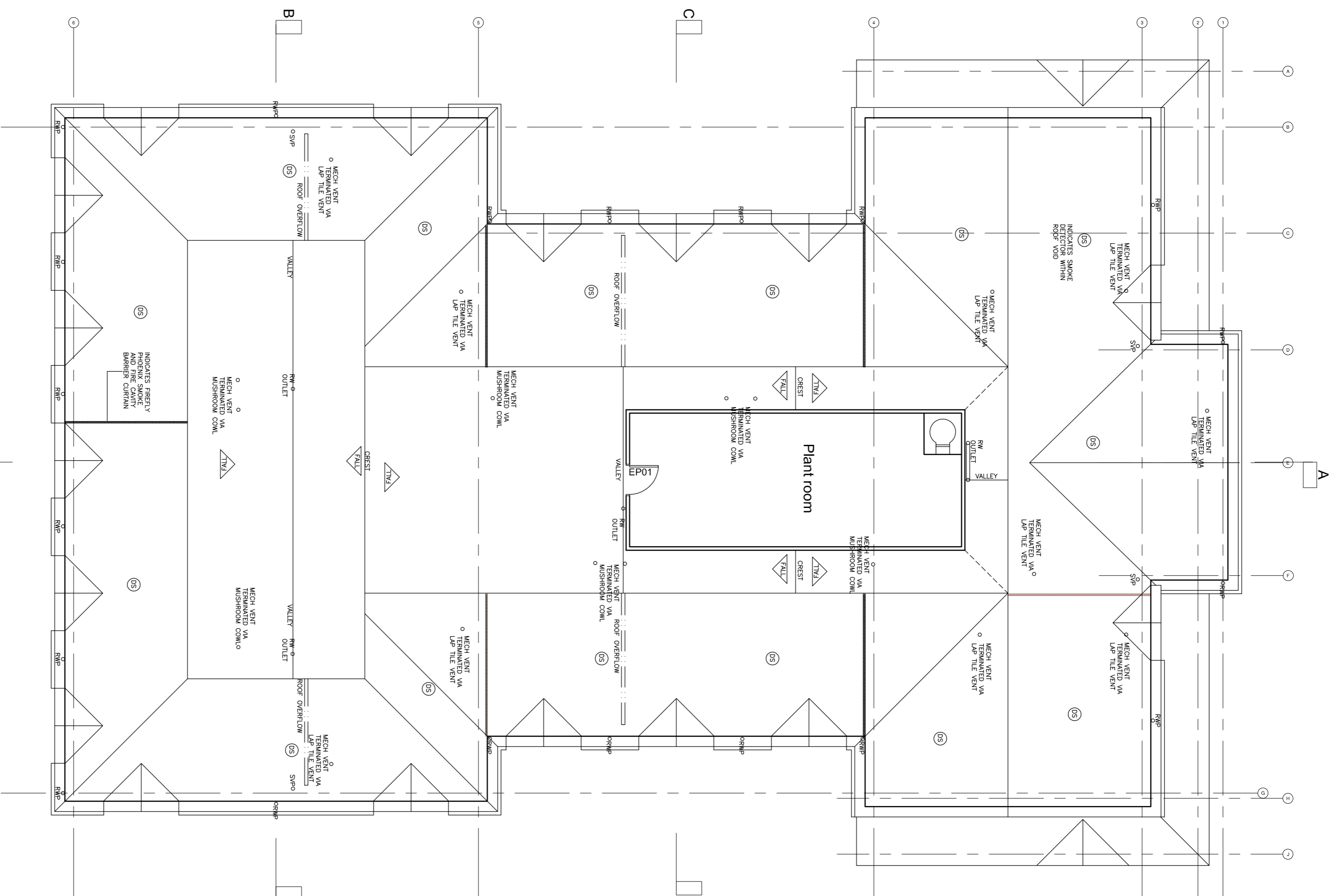
Roof Floor Plan
