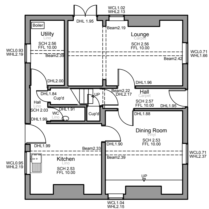
Ground Floor Plan 1:100 - A1
