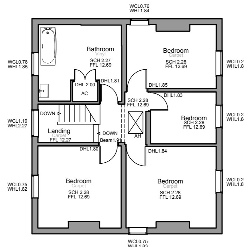
First Floor Plan 1:100 - A1
