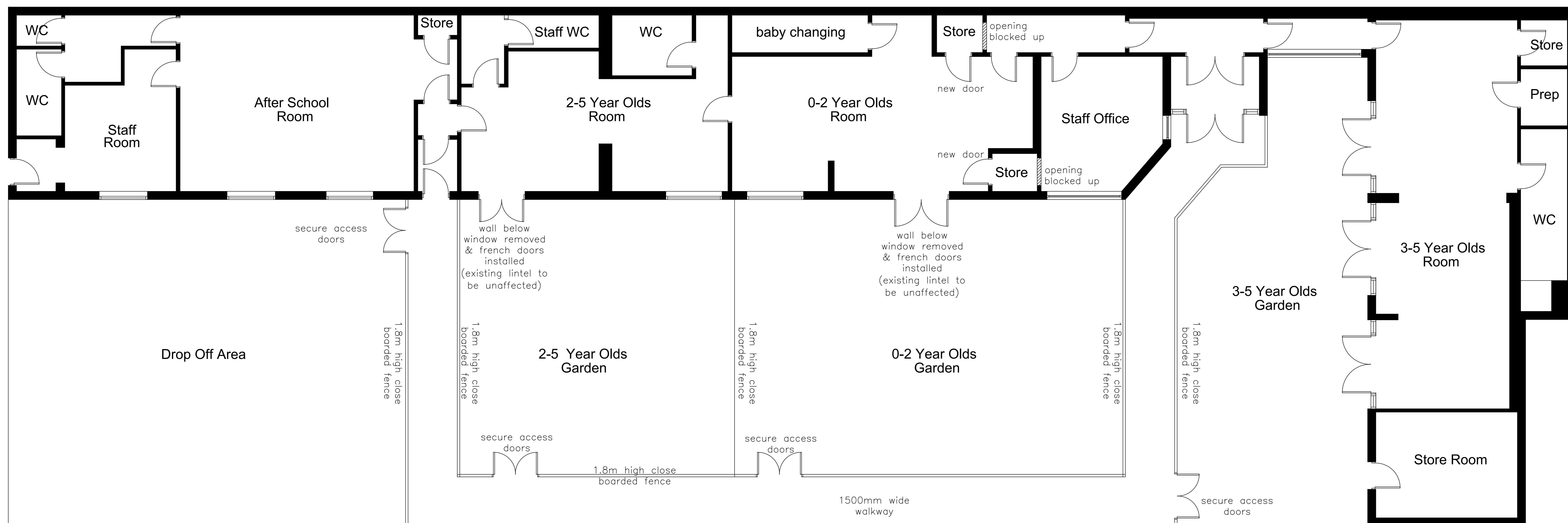
Proposed Plan 1:50
