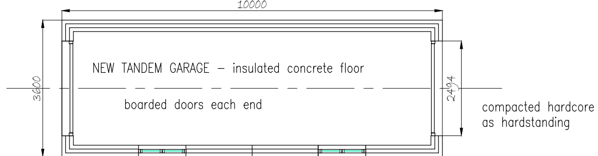
PROPOSED GF PLAN
