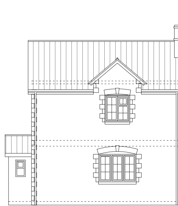
FRONT ELEVATION - 1:100
