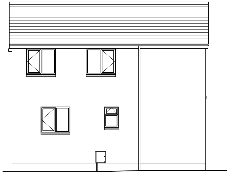
Front elevation, North
