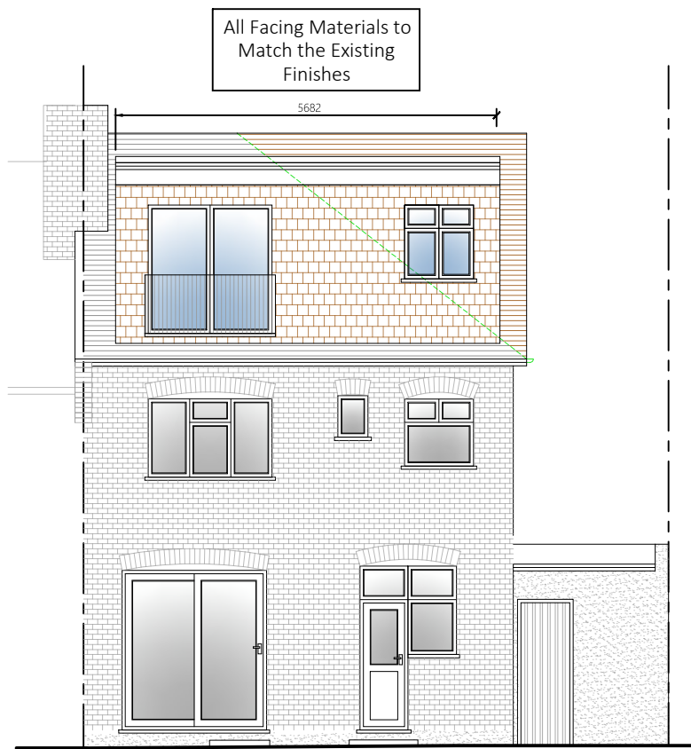
15 Proposed Rear Elevation SCALE: 1/100
