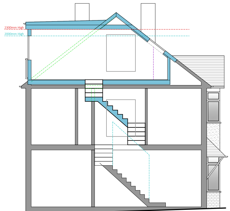
17 Proposed Side Section SCALE: 1/100
