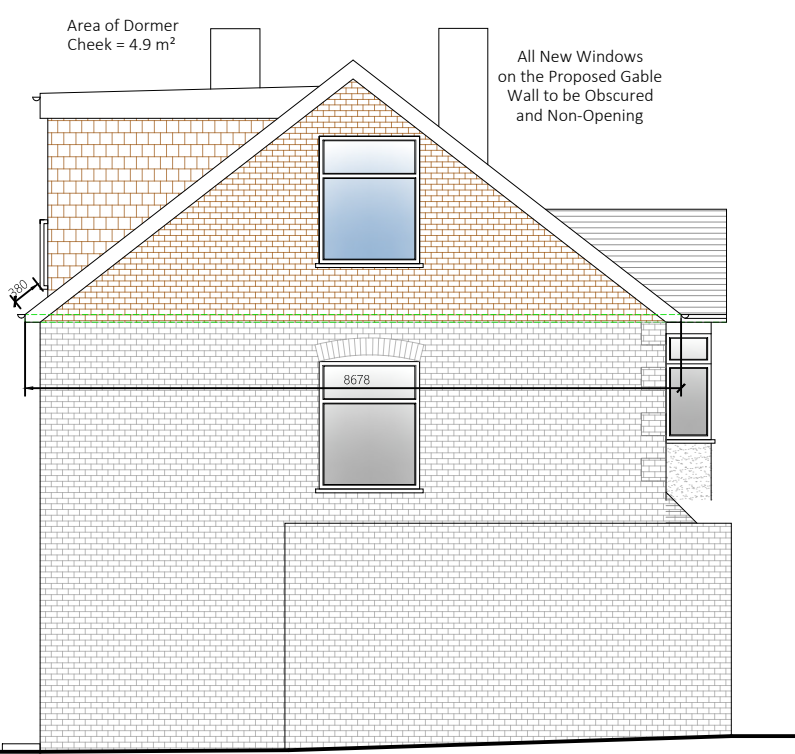
14 Proposed Side Elevation SCALE: 1/100
