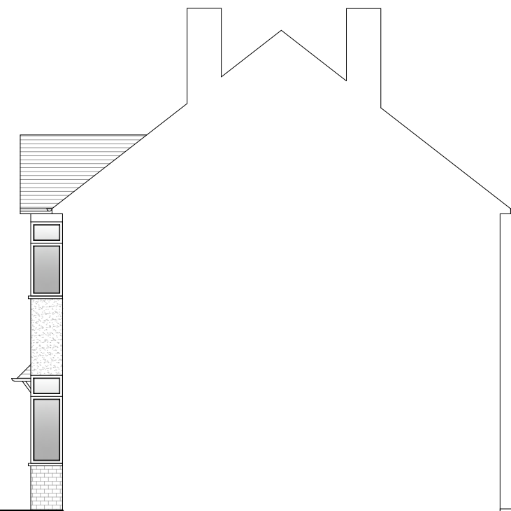
7 Existing Side Elevation SCALE: 1/100
