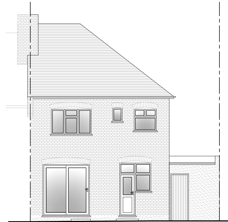
6 Existing Rear Elevation SCALE: 1/100
