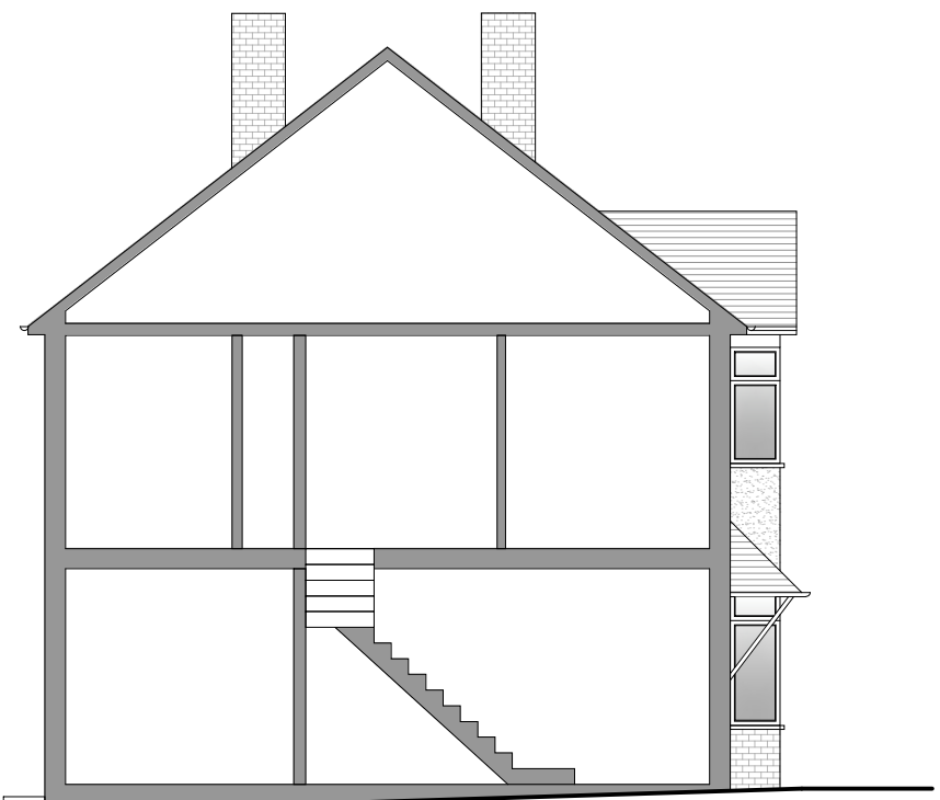
8 Existing Side Section SCALE: 1/100
