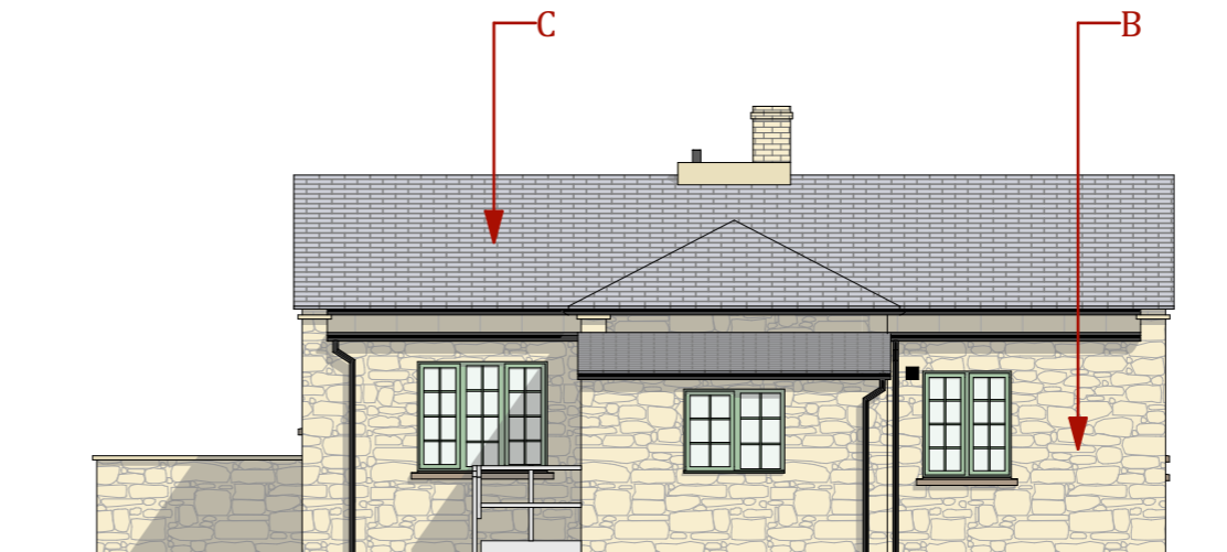
North Elevation
