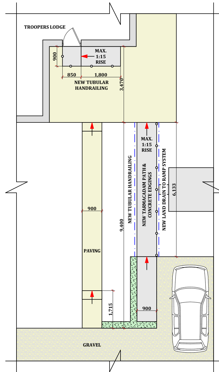
Ground Floor Plan (Proposed) - 1:100
