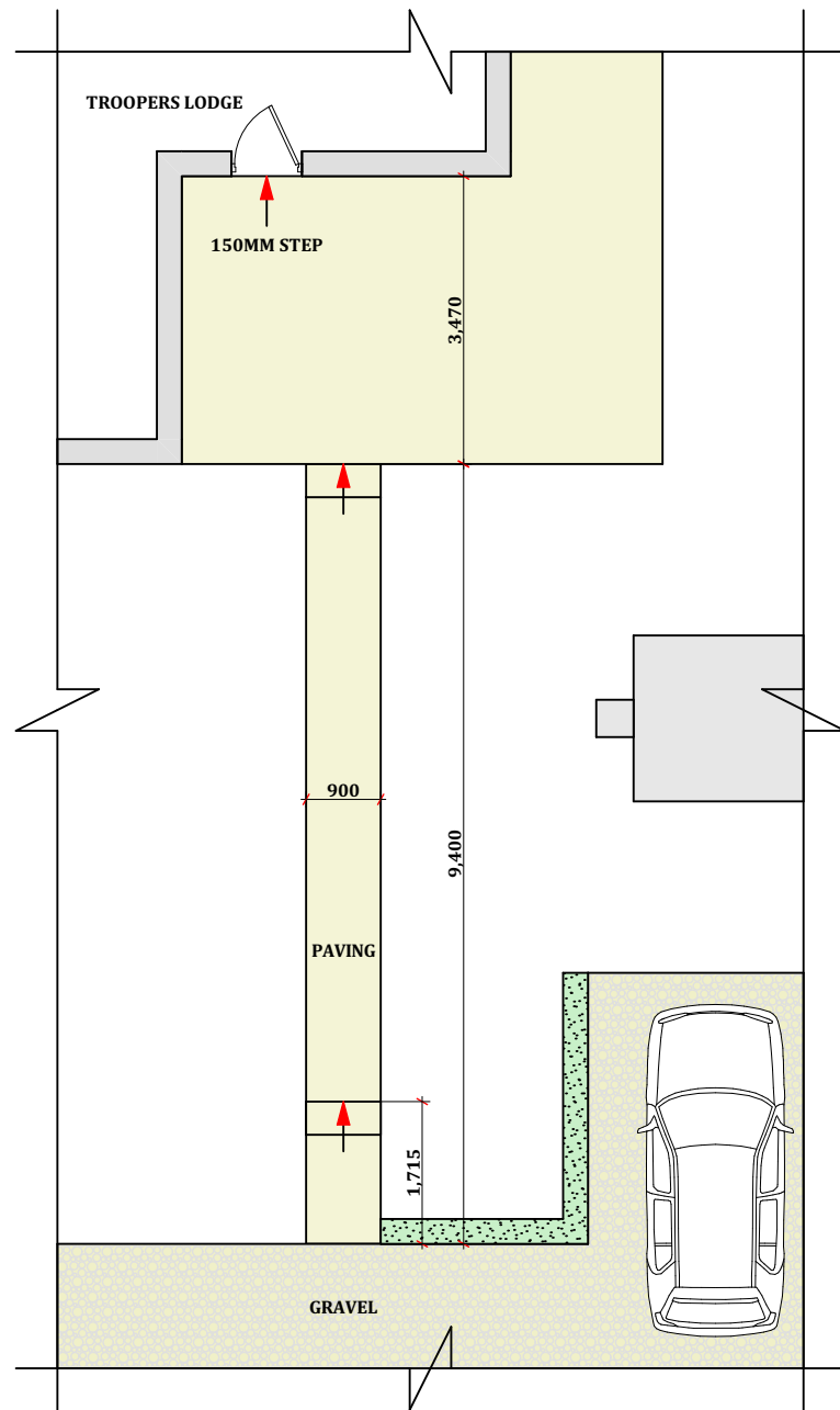
Ground Floor Plan (Existing) - 1:100
