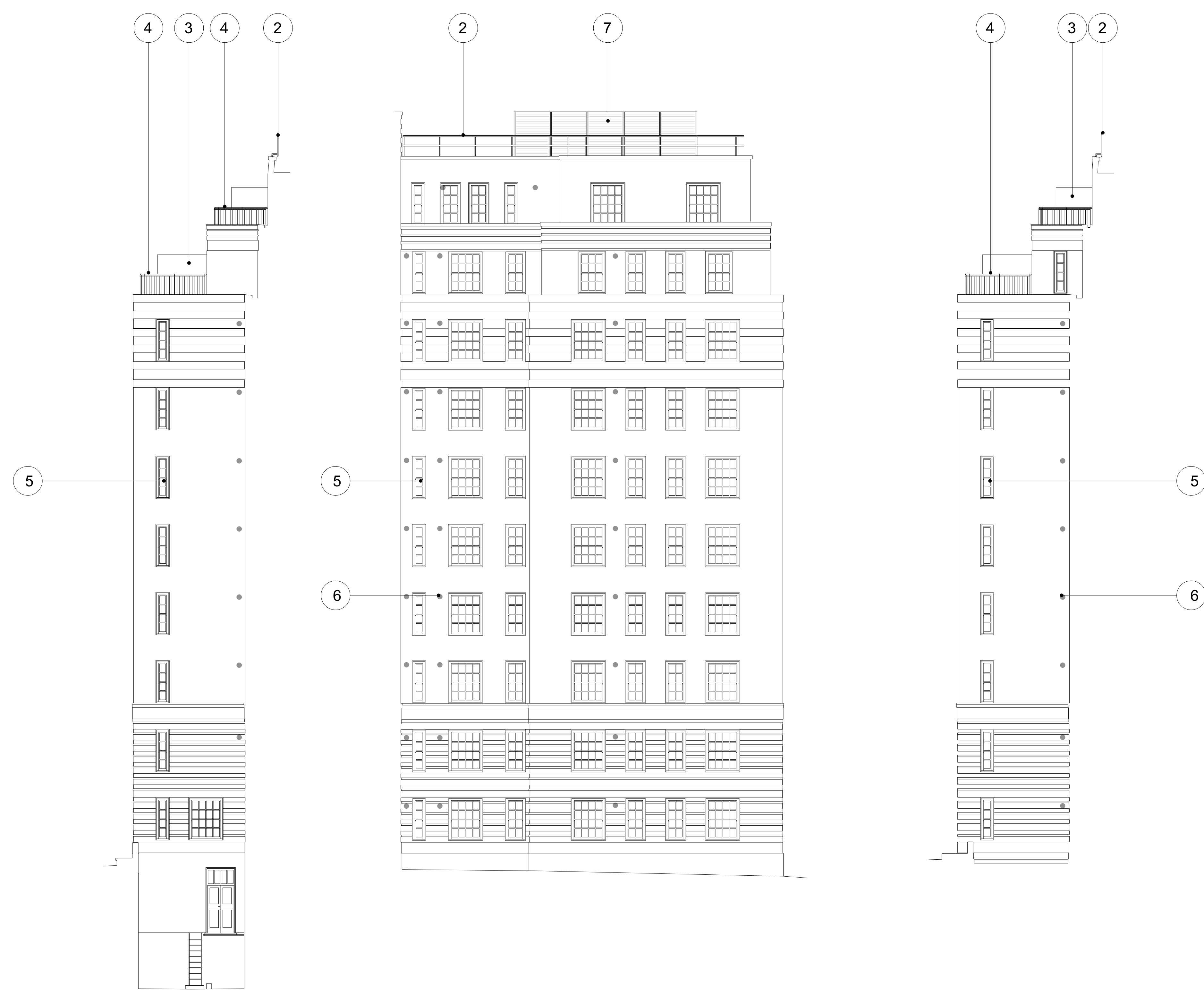
01 Howard House Proposed Elevation E-41 1:100
