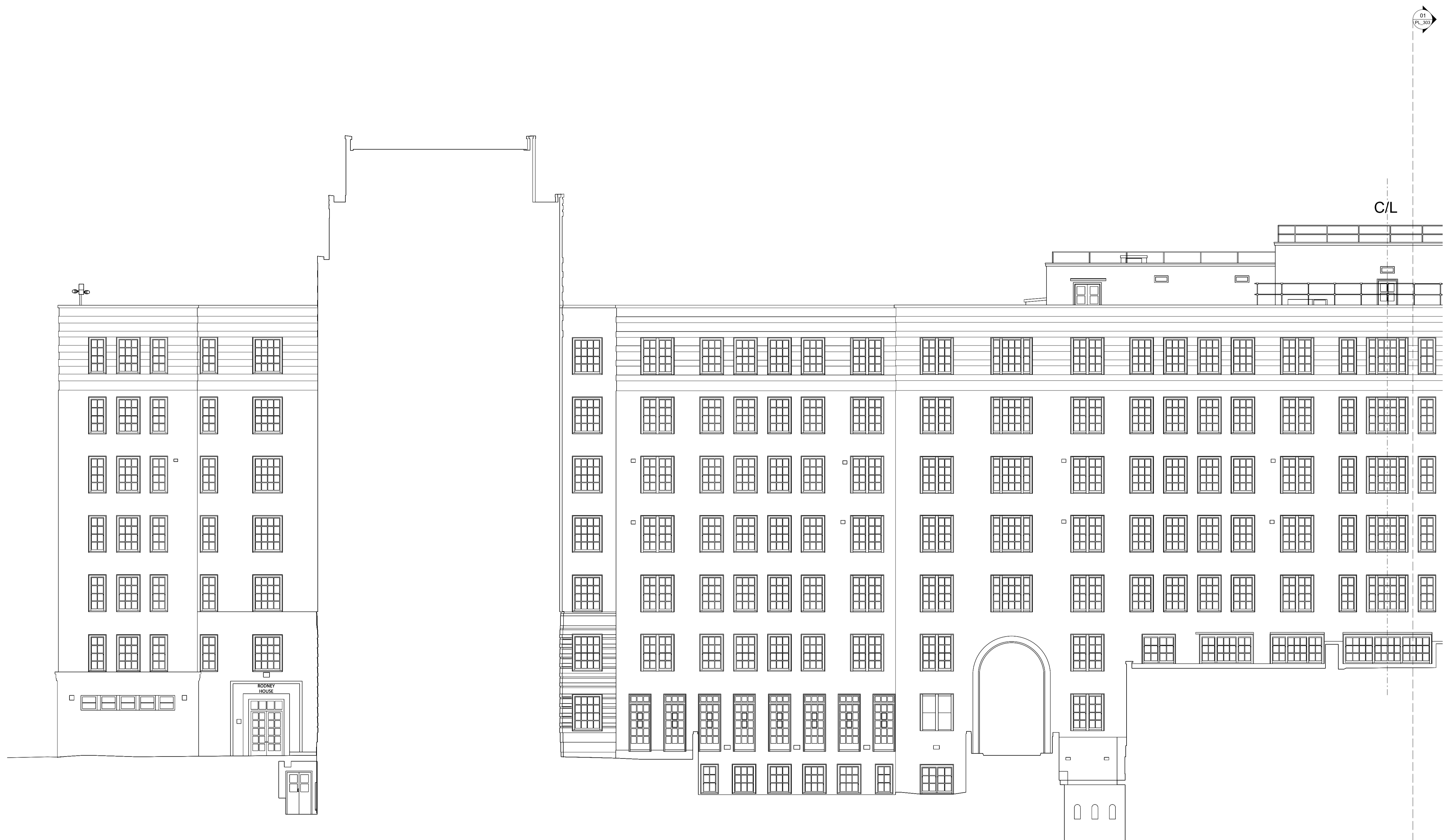
01 Rodney House Existing Elevation E-55 1:100
