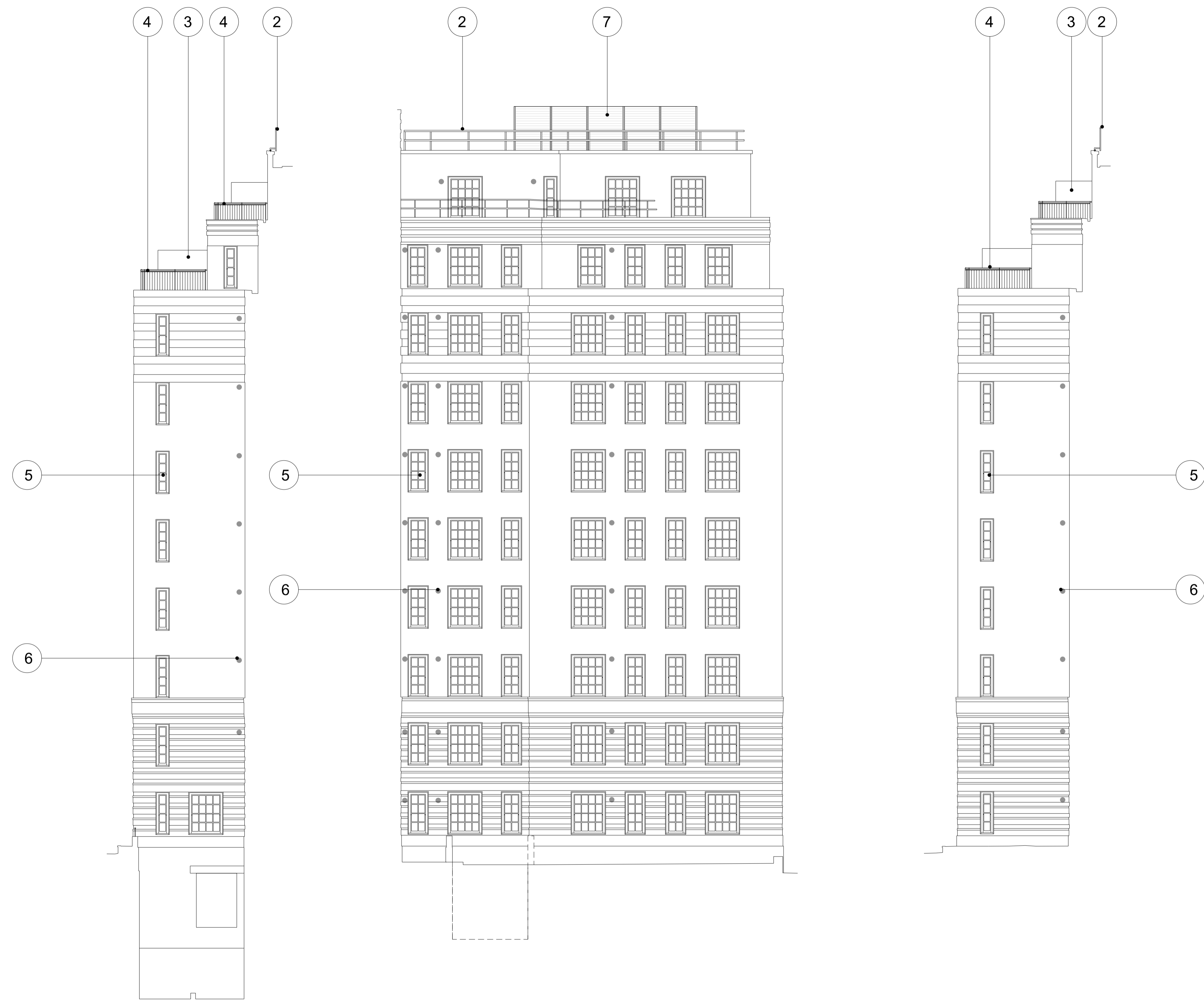
01 Hood House Proposed Elevation E-17 1:100
