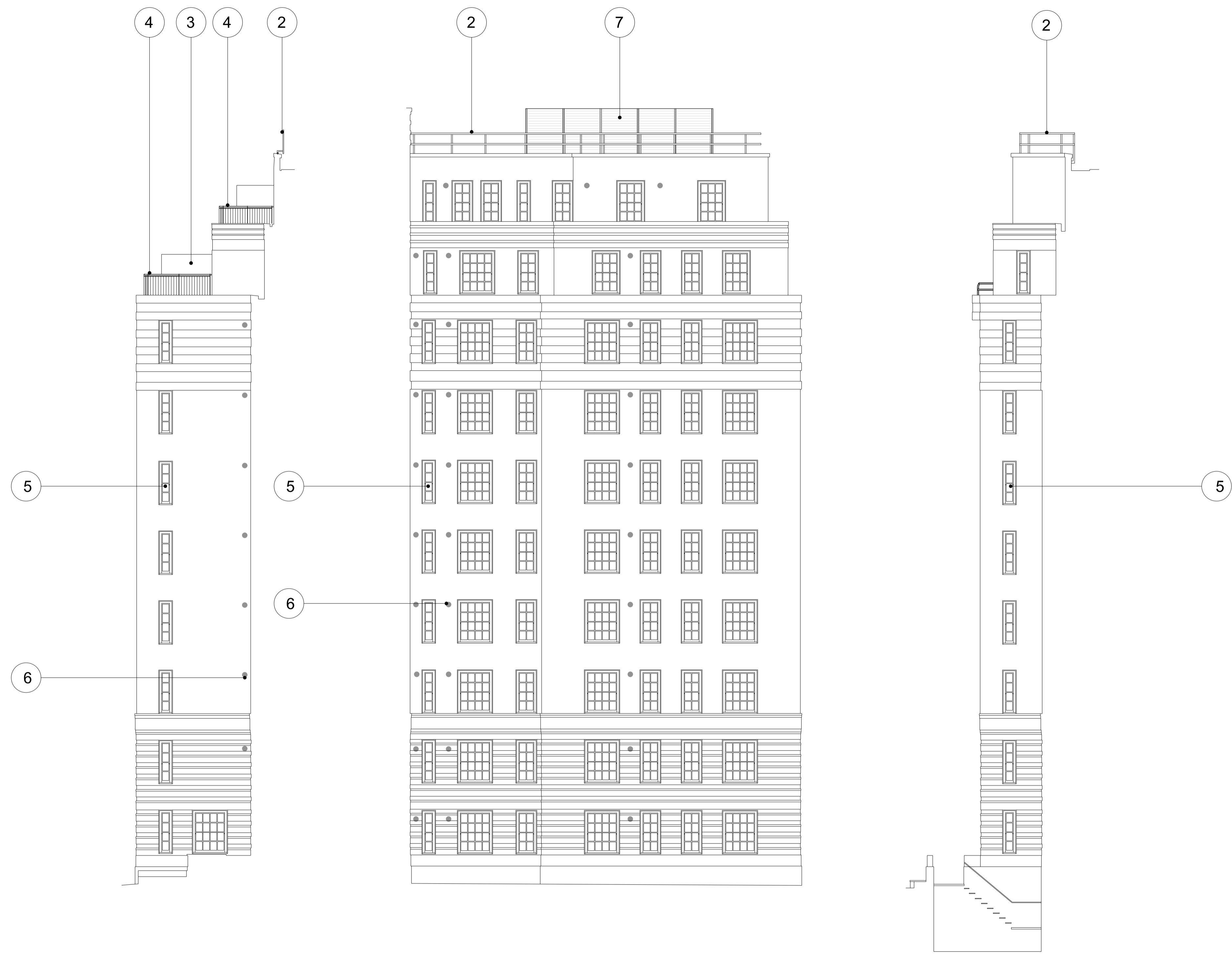
01 Frobisher House Proposed Elevation E-27 1:100
