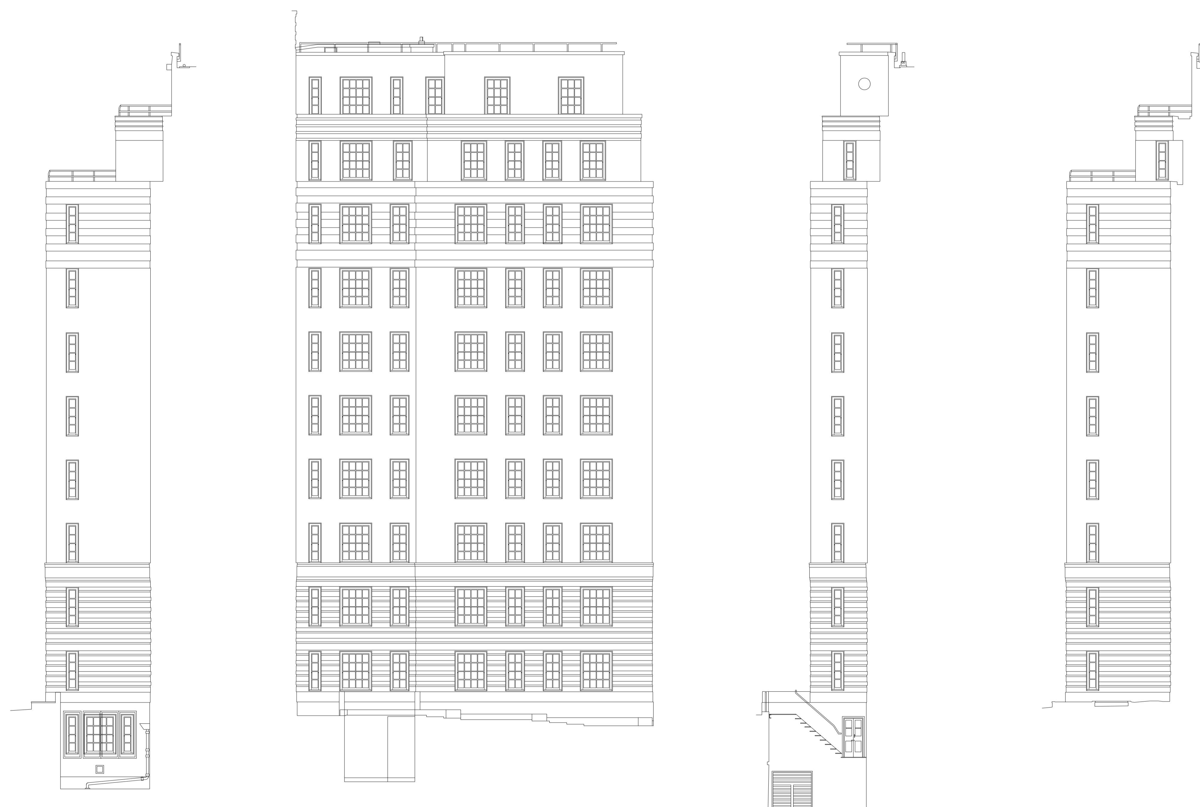
01 Collingwood House Existing Elevation E-23 1:100
