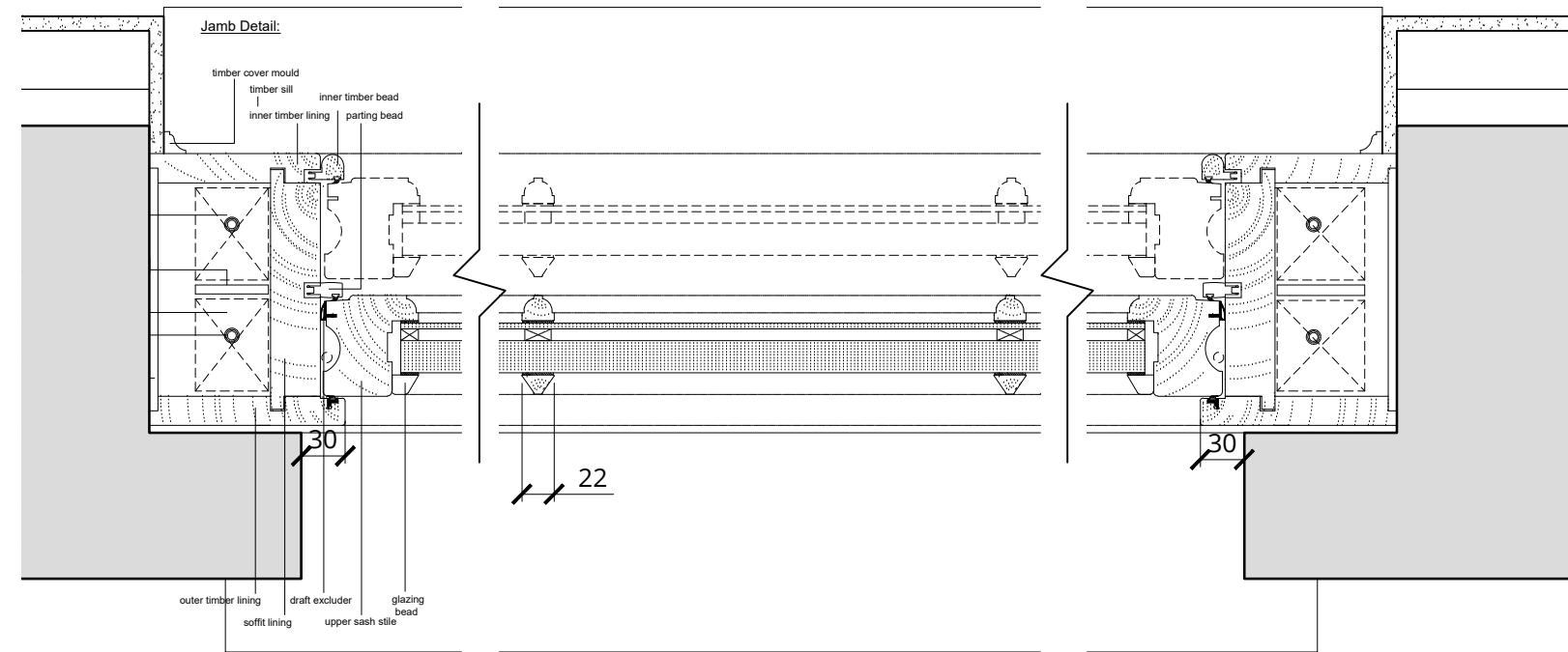
Typical Plan Scale 1:5
