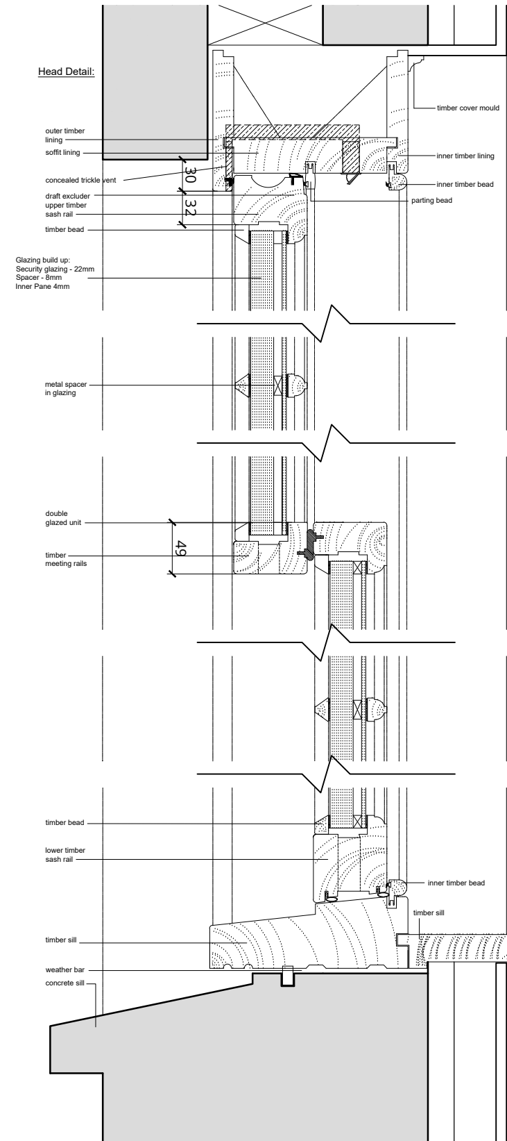
Typical Section Scale 1:5
