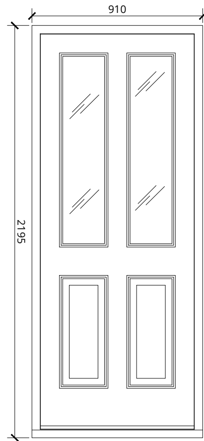
Typical Elevation Scale 1:20
