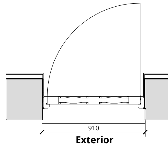
Typical Plan Scale 1:20
