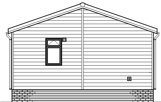
Front End Elevation
