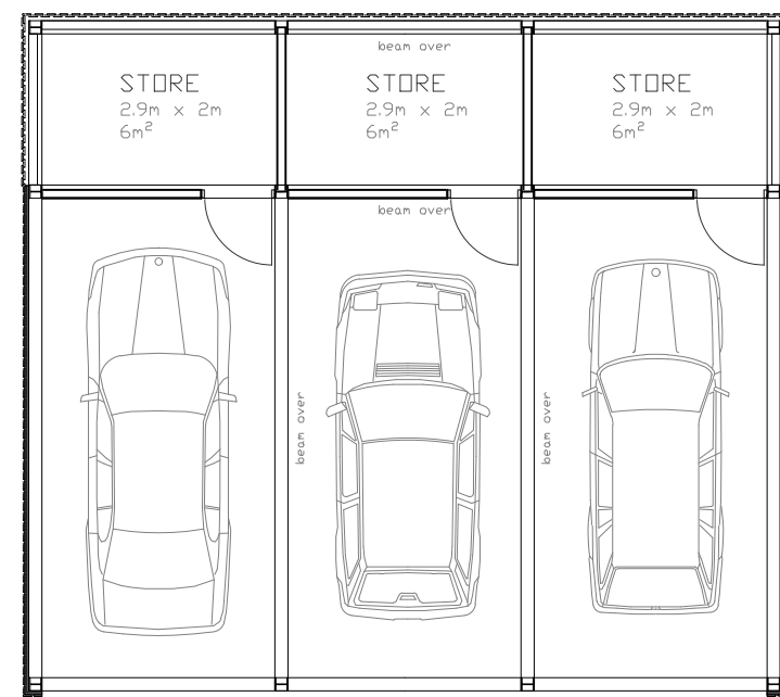
CARPORT 2 (PLOT 4)
