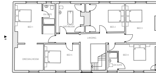
FIRST FLOOR PLAN (1:100)
