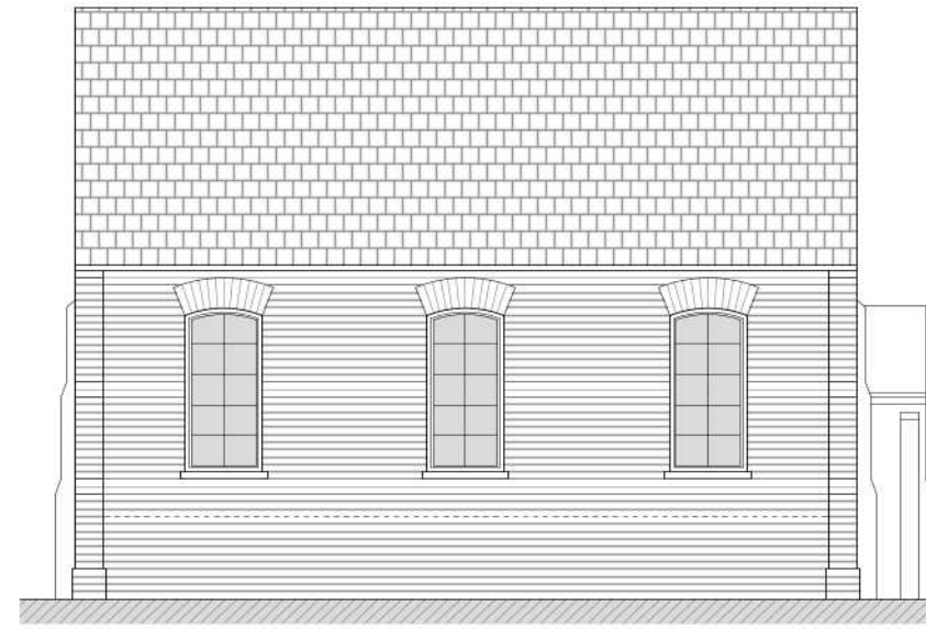
SIDE / WEST ELEVATION
