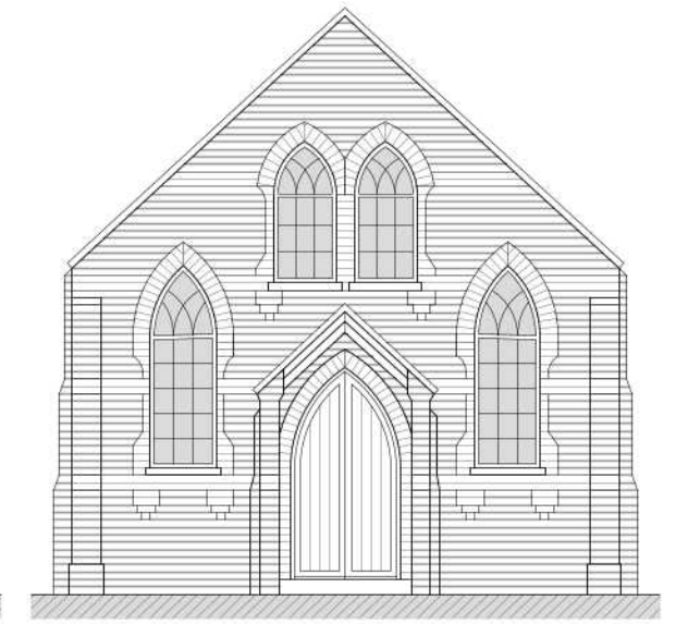
FRONT / SOUTH ELEVATION
