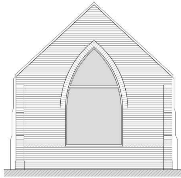
REAR / NORTH ELEVATION
