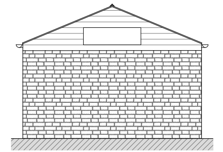
South Elevation
