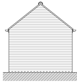
West Elevation
