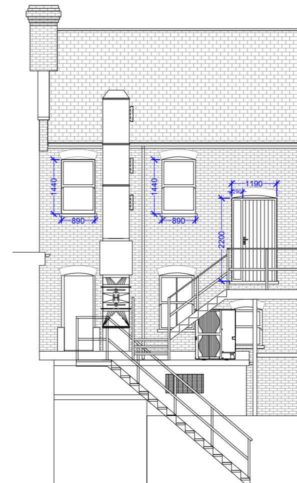
04 REAR ELEVATION 1:100
