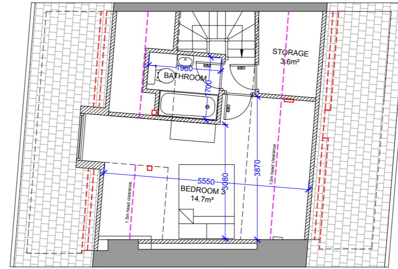
01 ATTIC PLAN 1:100
