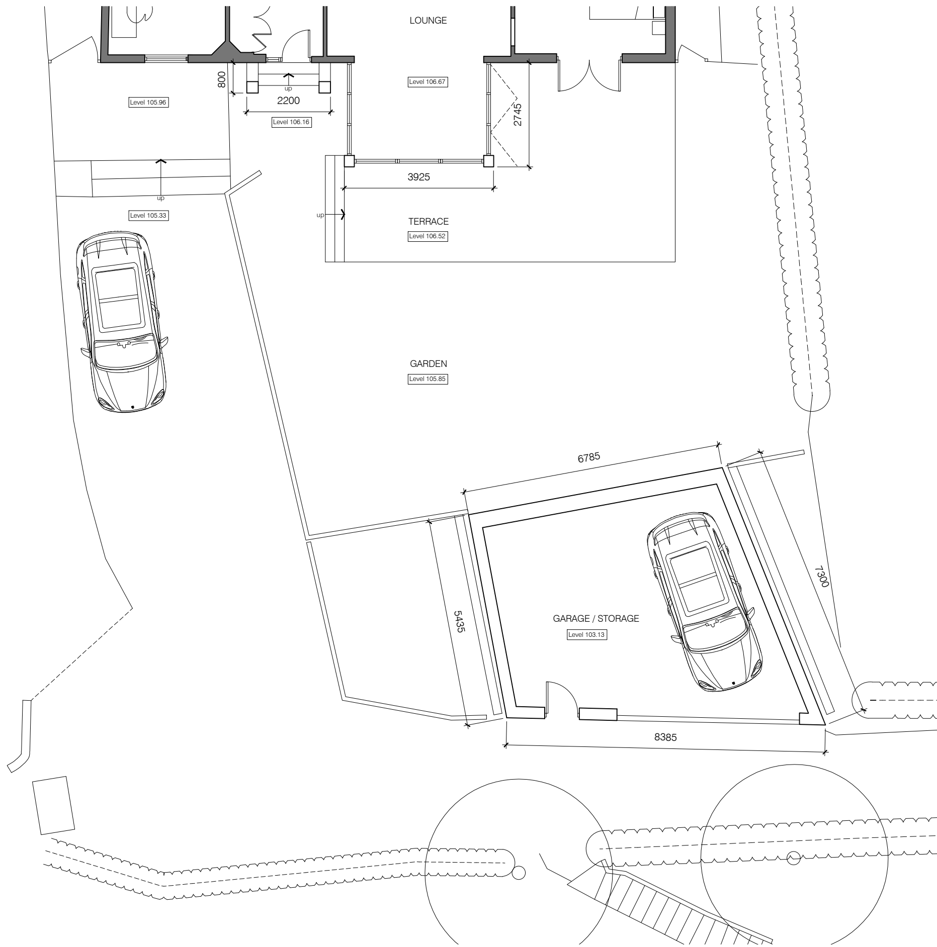
PROPOSED GROUND FLOOR PLAN - GARAGE
