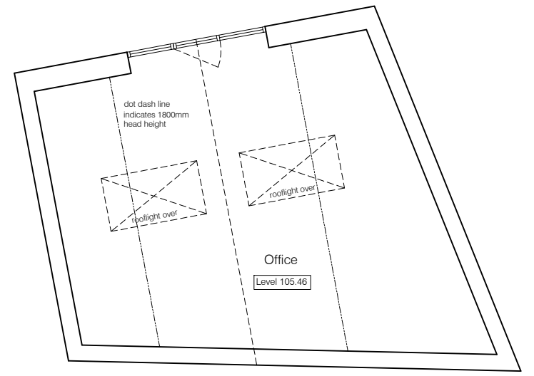
PROPOSED FIRST FLOOR PLAN - GARAGE
