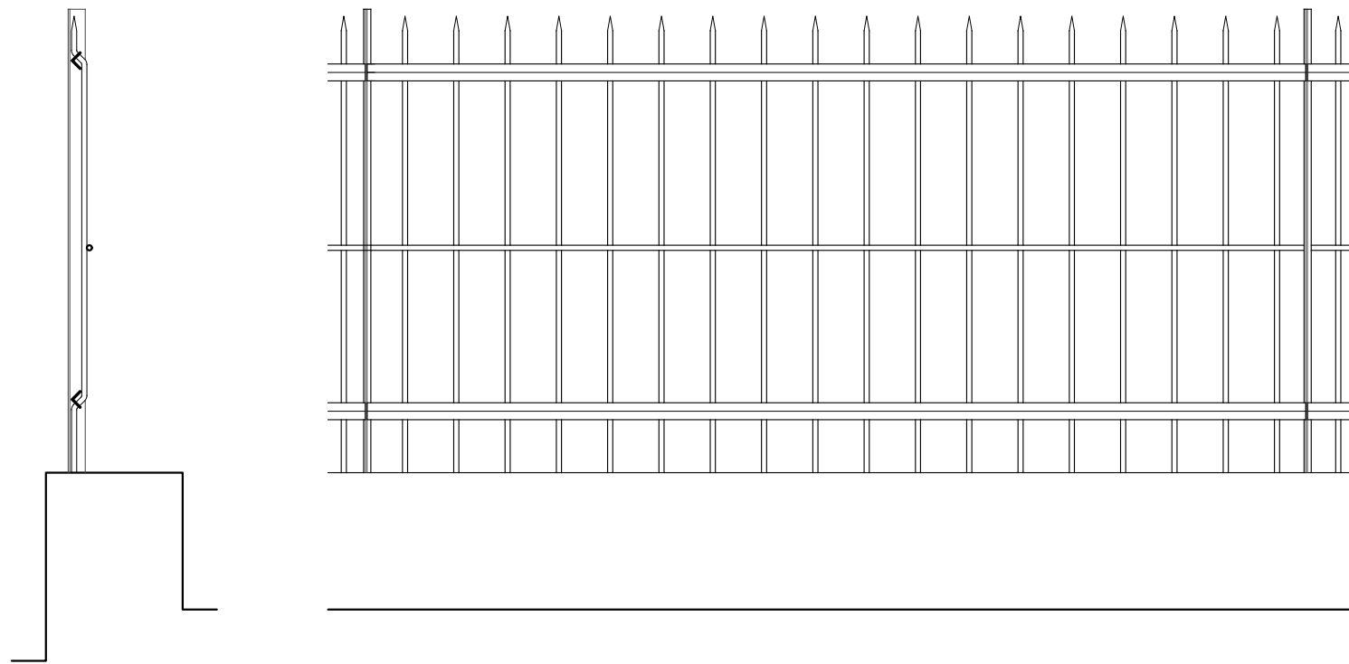
Existing Section and Elevation - 1:20
