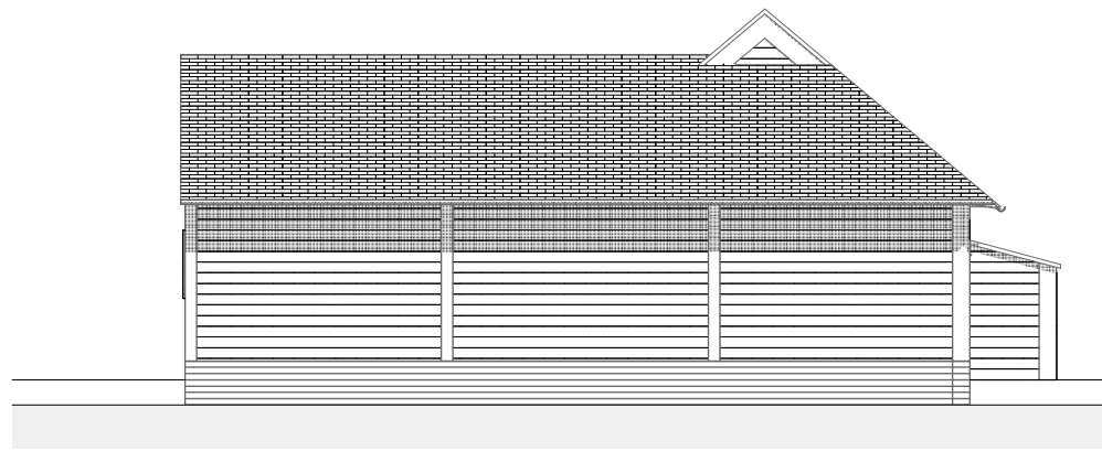
4 Side Elevation Two 1:100
