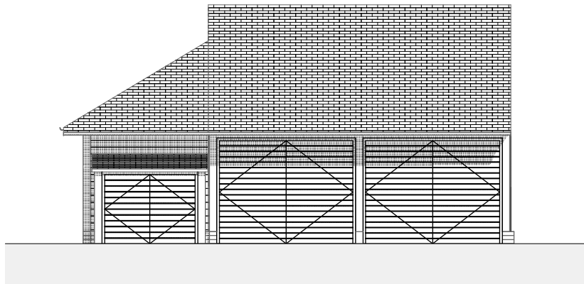
1 Front Elevation 1:100
