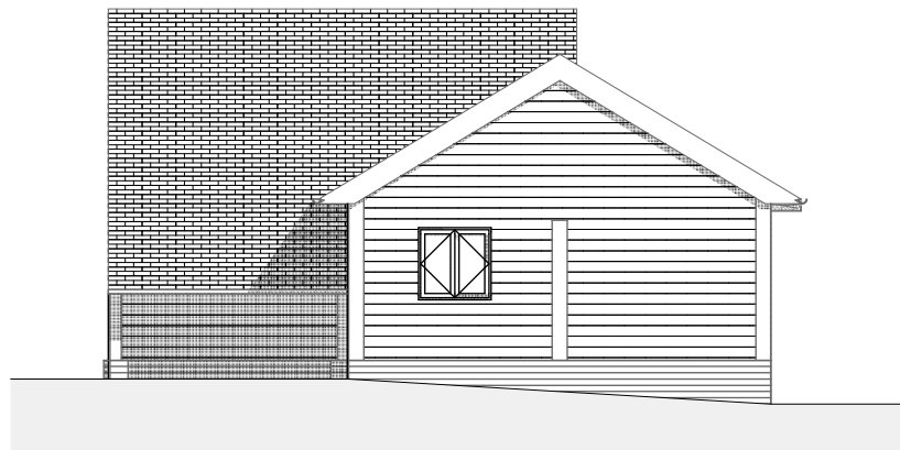
3 Rear Elevation 1:100
