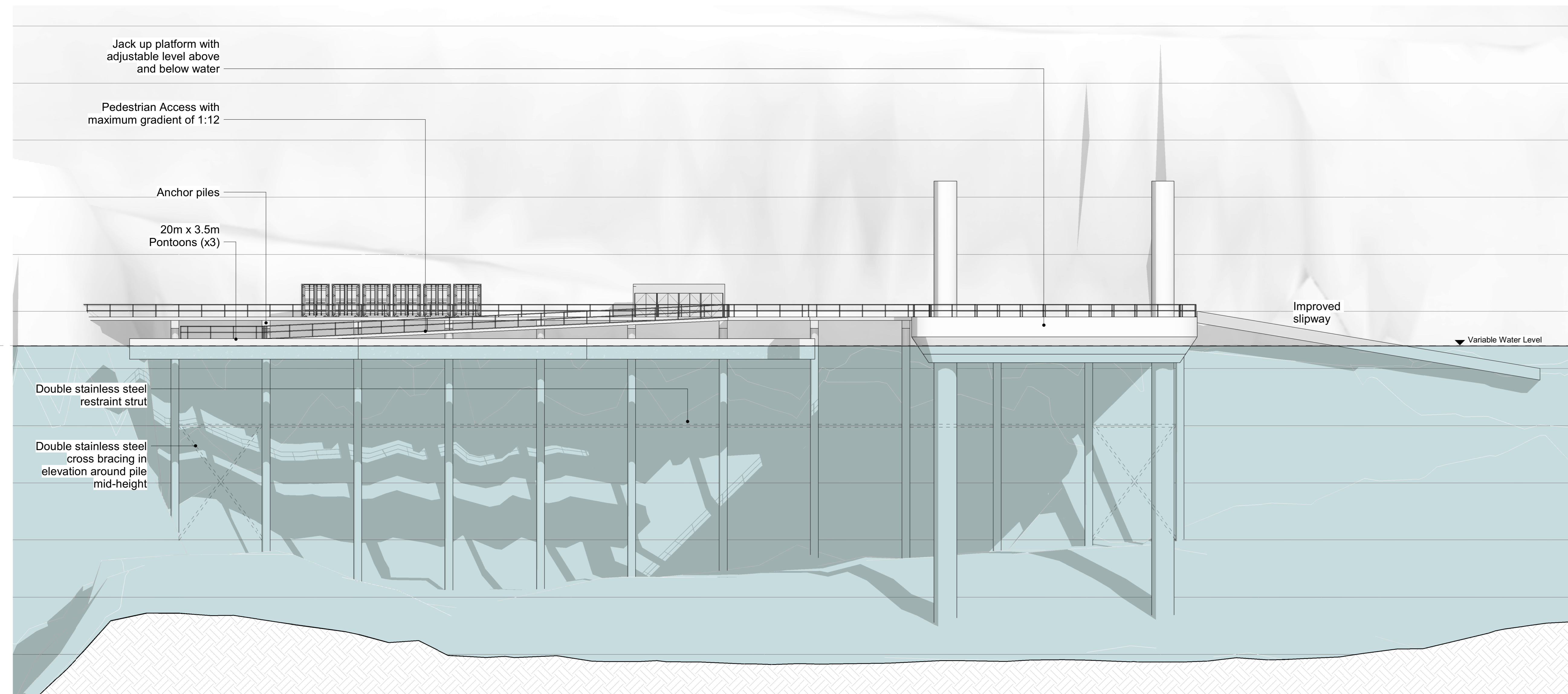
2 Section 1 - Apron & Jack Up Platform 1 : 200
