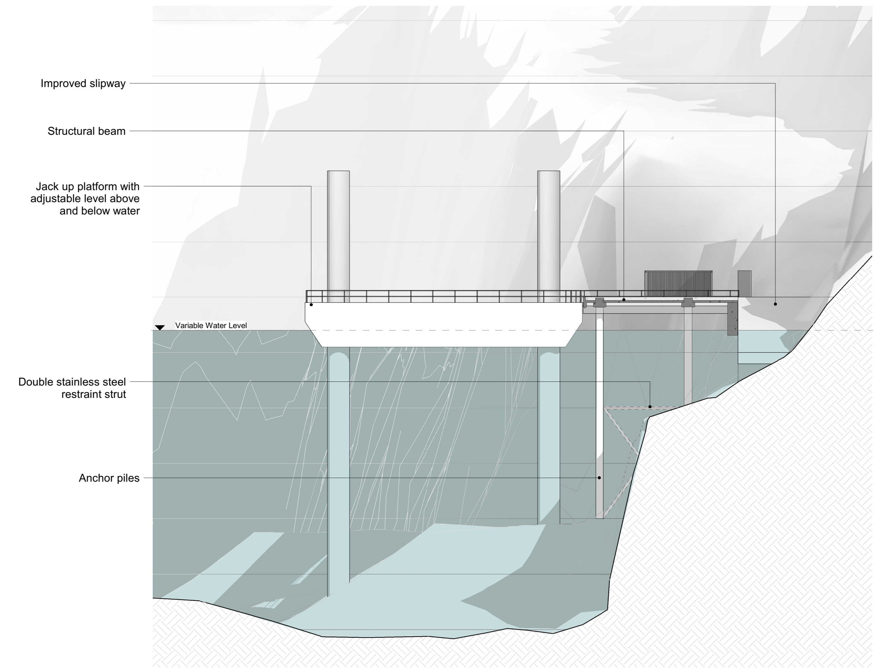
4 Section 3 - Apron & Jack Up Platform 1 : 200
