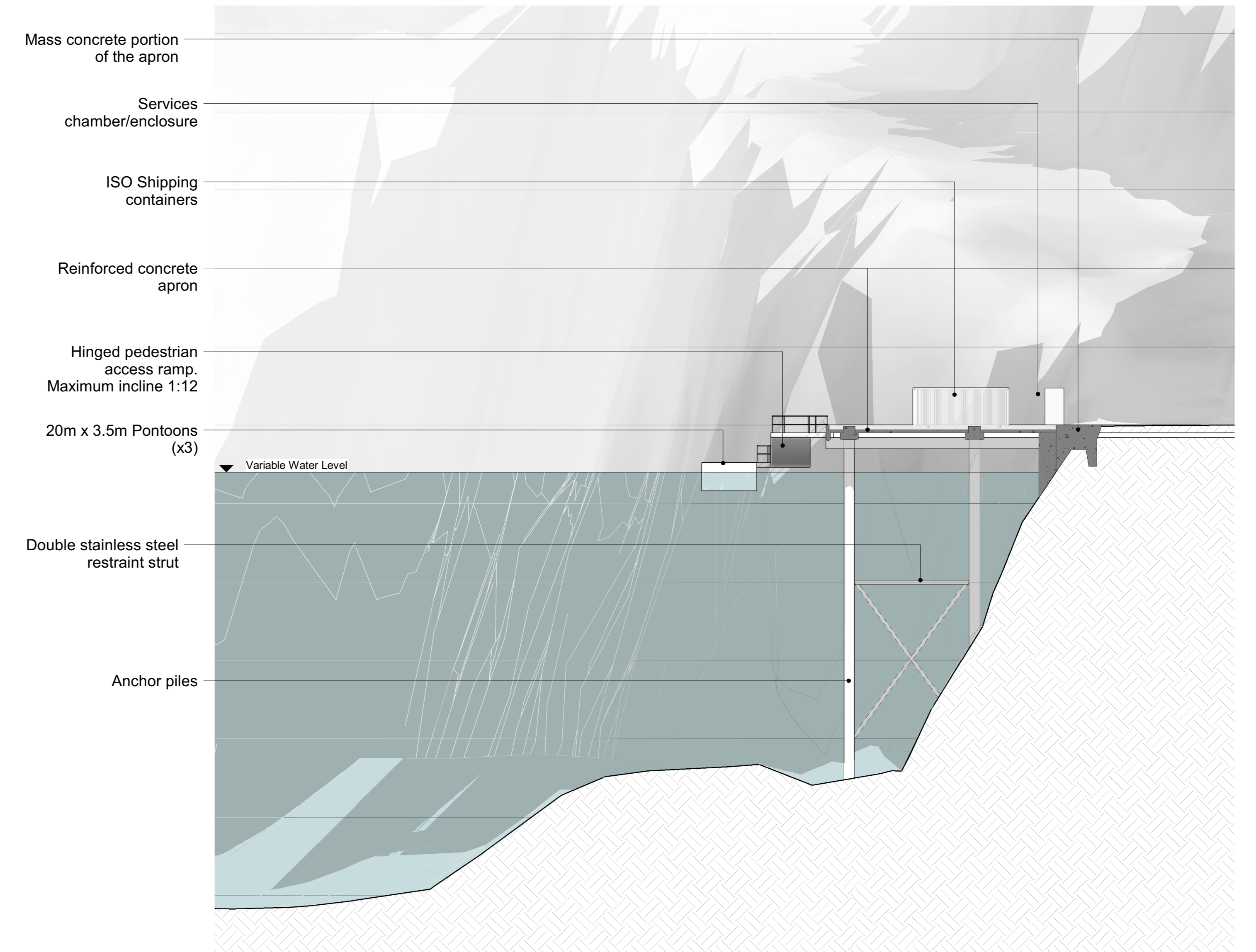
3 Section 2 - Apron & Jack Up Platform 1 : 200
