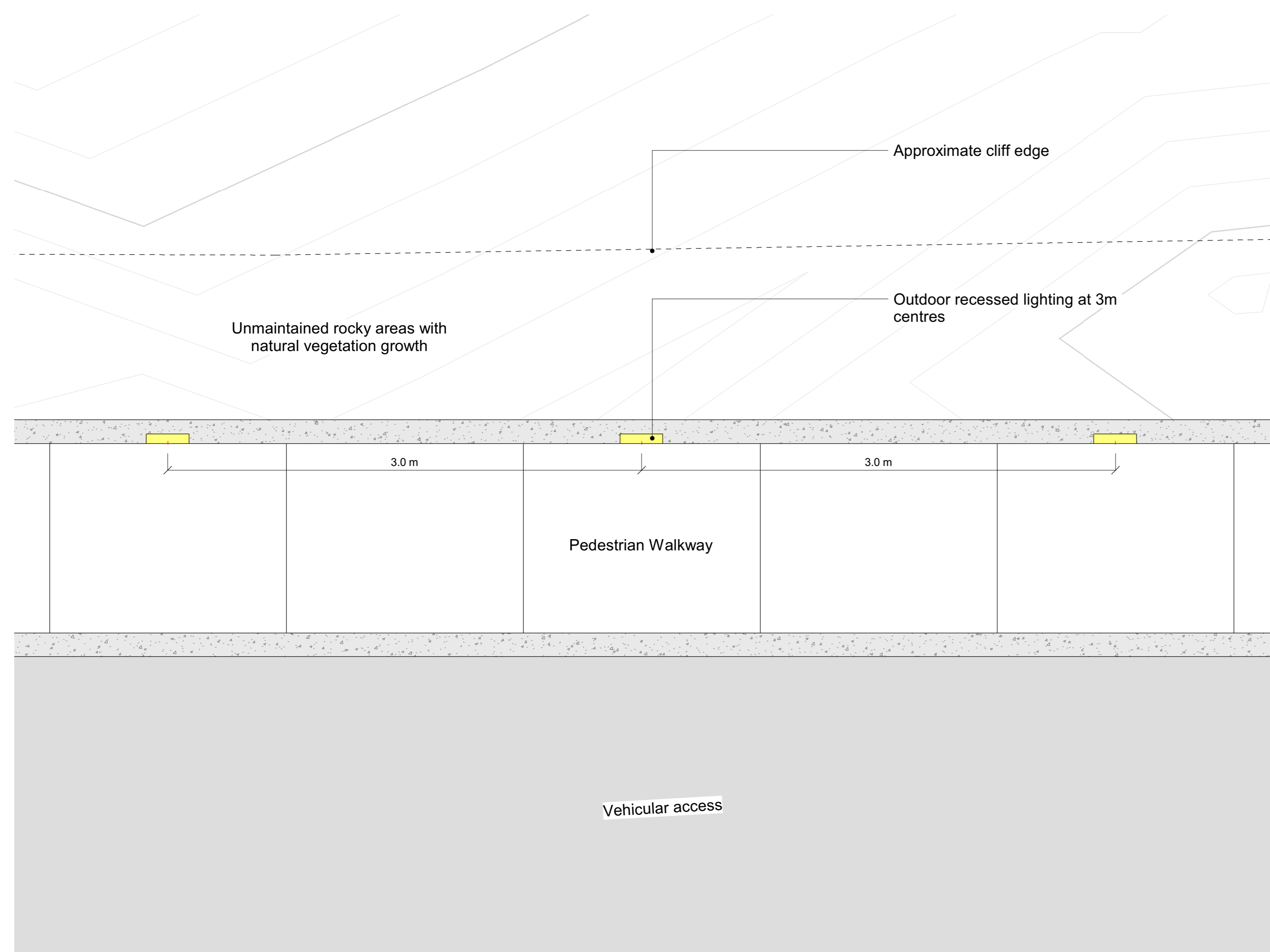
1 PL_P_420_Quarry Haul Road Typical Lighting Plan 1 : 20
