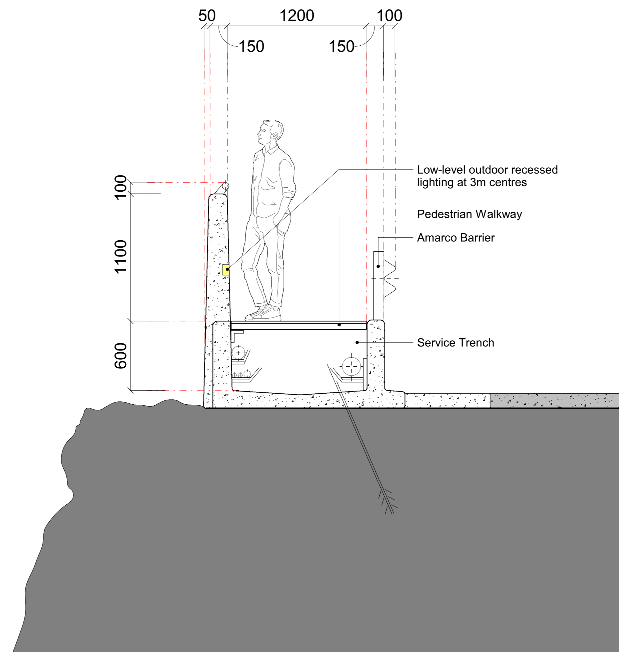
2 PL_Quarry Access Road_Detailed Section Lighting 1 : 20
