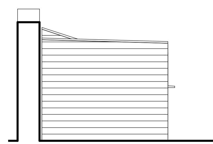
4 01.A1 EXISTING WEST ELEVATION 1 : 50
